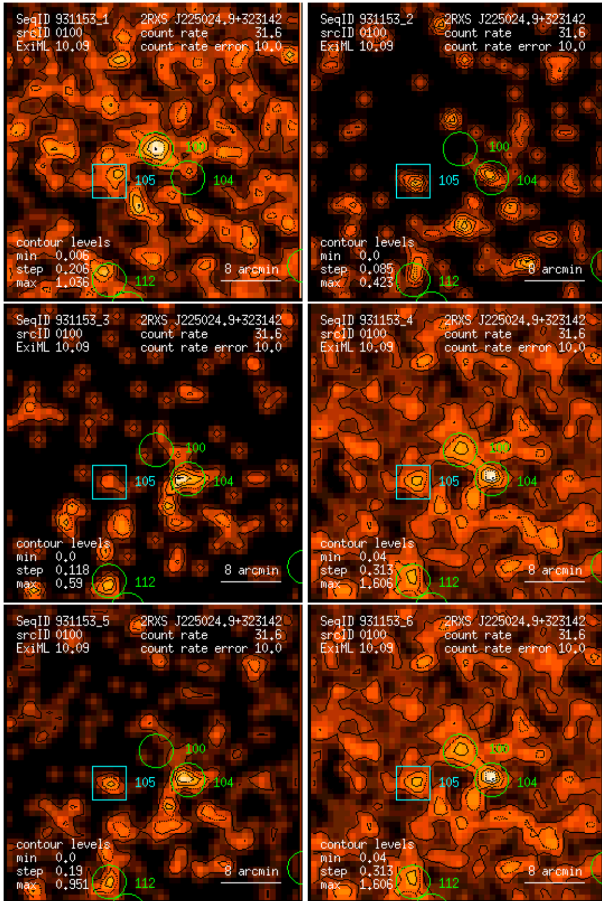
Figure 100: RASS 931153: detection 0100: band rate images, Gaussian filter: (1) PSPC channels 11 – 41, (2) 52 – 90, (3) 91 – 201, (4) 11 – 235, (5) 52 – 201, (6) 11 – 201. Broad band rates in counts/ks. Band rate contour levels in counts/ks/arcmin 2 .
