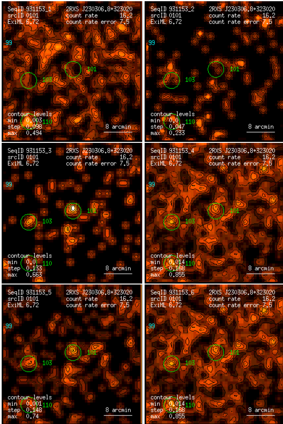
Figure 101: RASS 931153: detection 0101: band rate images, Gaussian filter: (1) PSPC channels 11 – 41, (2) 52 – 90, (3) 91 – 201, (4) 11 – 235, (5) 52 – 201, (6) 11 – 201. Broad band rates in counts/ks. Band rate contour levels in counts/ks/arcmin 2 .
