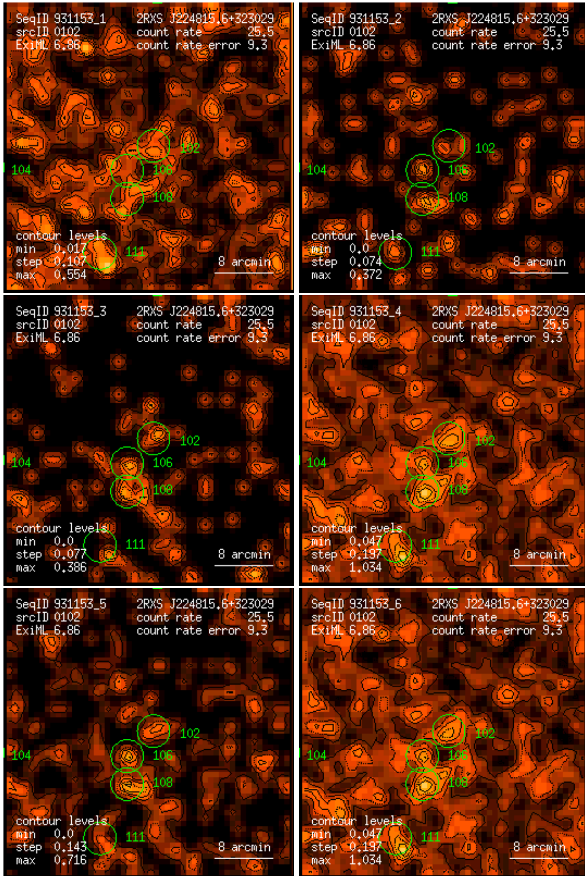
Figure 102: RASS 931153: detection 0102: band rate images, Gaussian filter: (1) PSPC channels 11 – 41, (2) 52 – 90, (3) 91 – 201, (4) 11 – 235, (5) 52 – 201, (6) 11 – 201. Broad band rates in counts/ks. Band rate contour levels in counts/ks/arcmin 2 .
