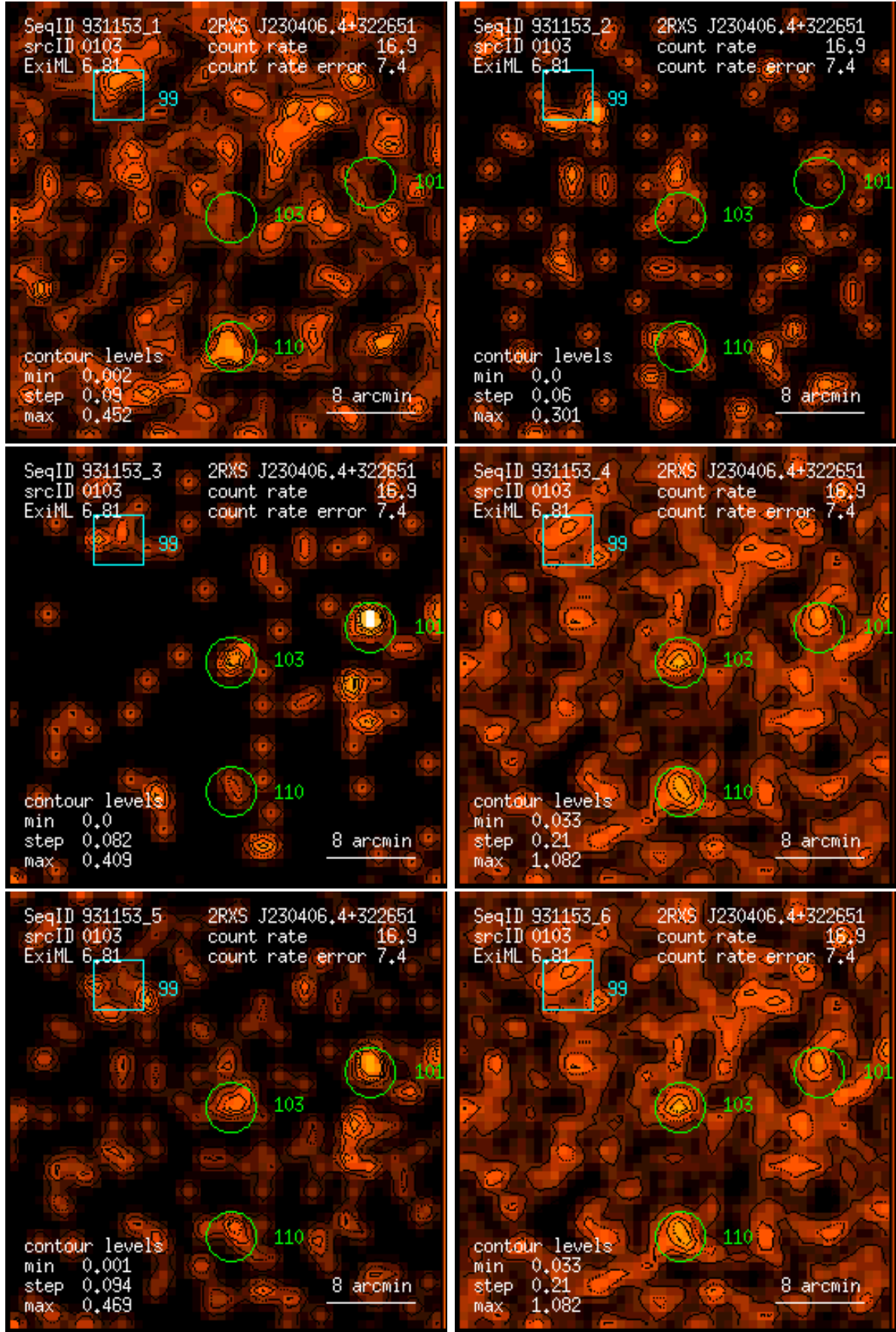
Figure 103: RASS 931153: detection 0103: band rate images, Gaussian filter: (1) PSPC channels 11 – 41, (2) 52 – 90, (3) 91 – 201, (4) 11 – 235, (5) 52 – 201, (6) 11 – 201. Broad band rates in counts/ks. Band rate contour levels in counts/ks/arcmin 2 .
