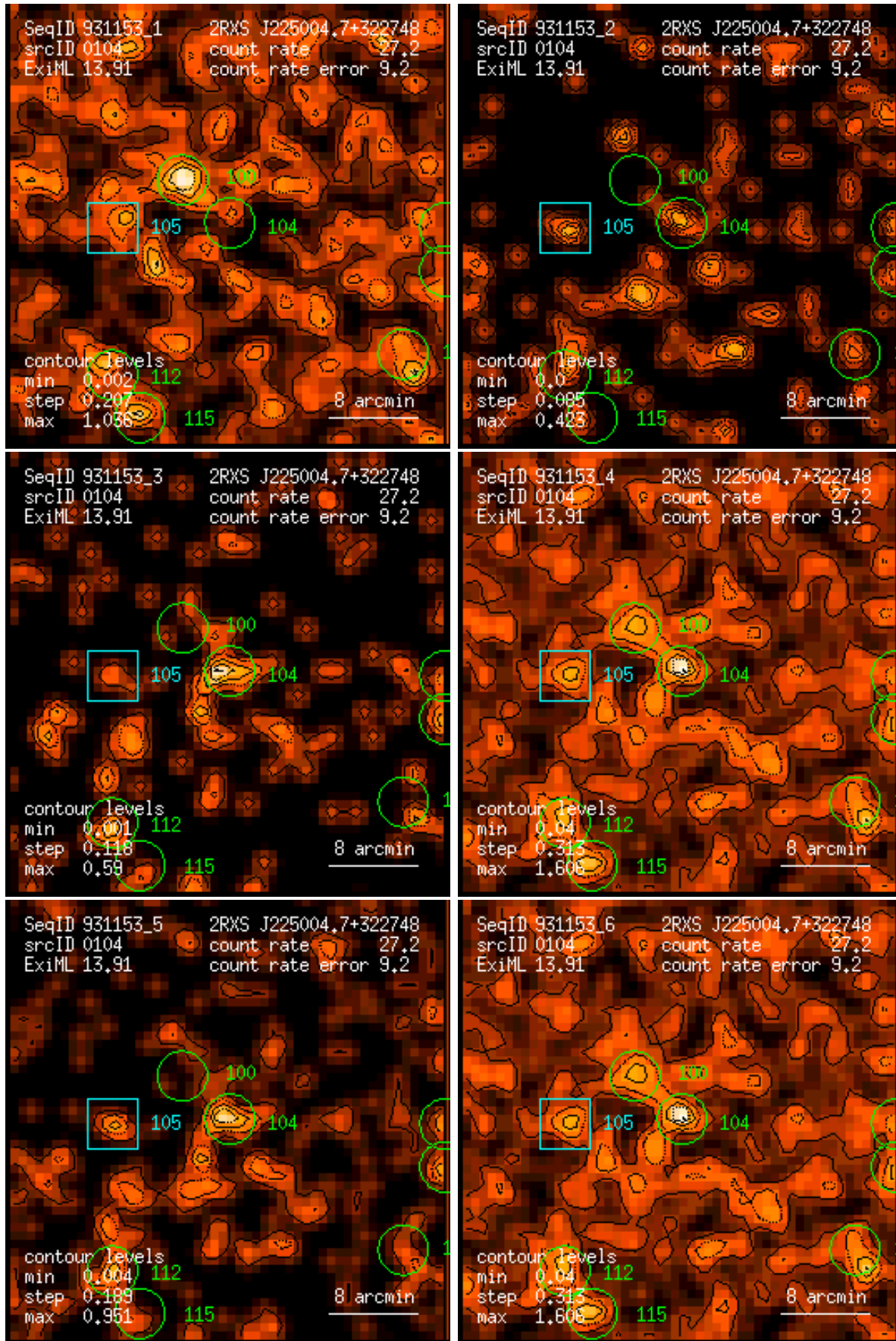
Figure 104: RASS 931153: detection 0104: band rate images, Gaussian filter: (1) PSPC channels 11 – 41, (2) 52 – 90, (3) 91 – 201, (4) 11 – 235, (5) 52 – 201, (6) 11 – 201. Broad band rates in counts/ks. Band rate contour levels in counts/ks/arcmin 2 .
