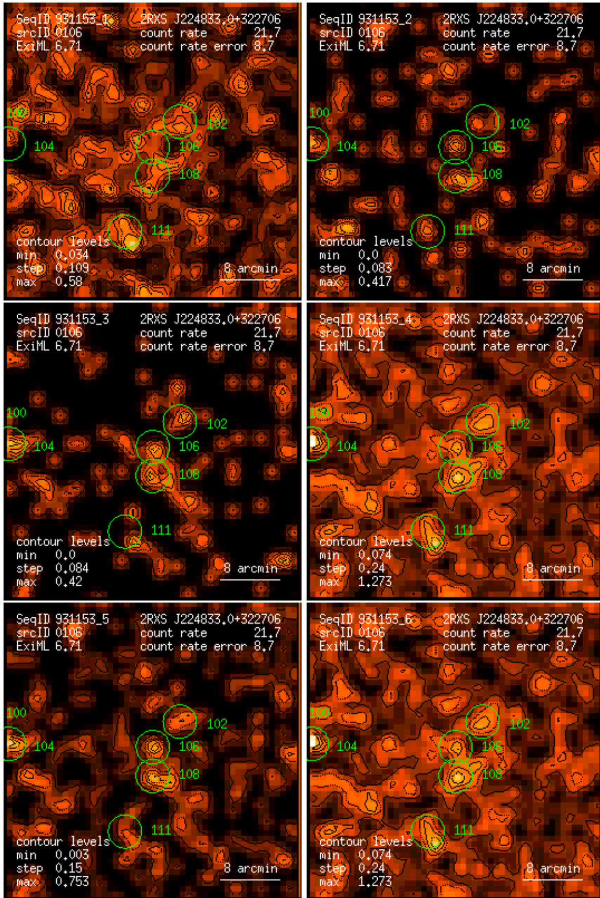
Figure 106: RASS 931153: detection 0106: band rate images, Gaussian filter: (1) PSPC channels 11 – 41, (2) 52 – 90, (3) 91 – 201, (4) 11 – 235, (5) 52 – 201, (6) 11 – 201. Broad band rates in counts/ks. Band rate contour levels in counts/ks/arcmin 2 .
