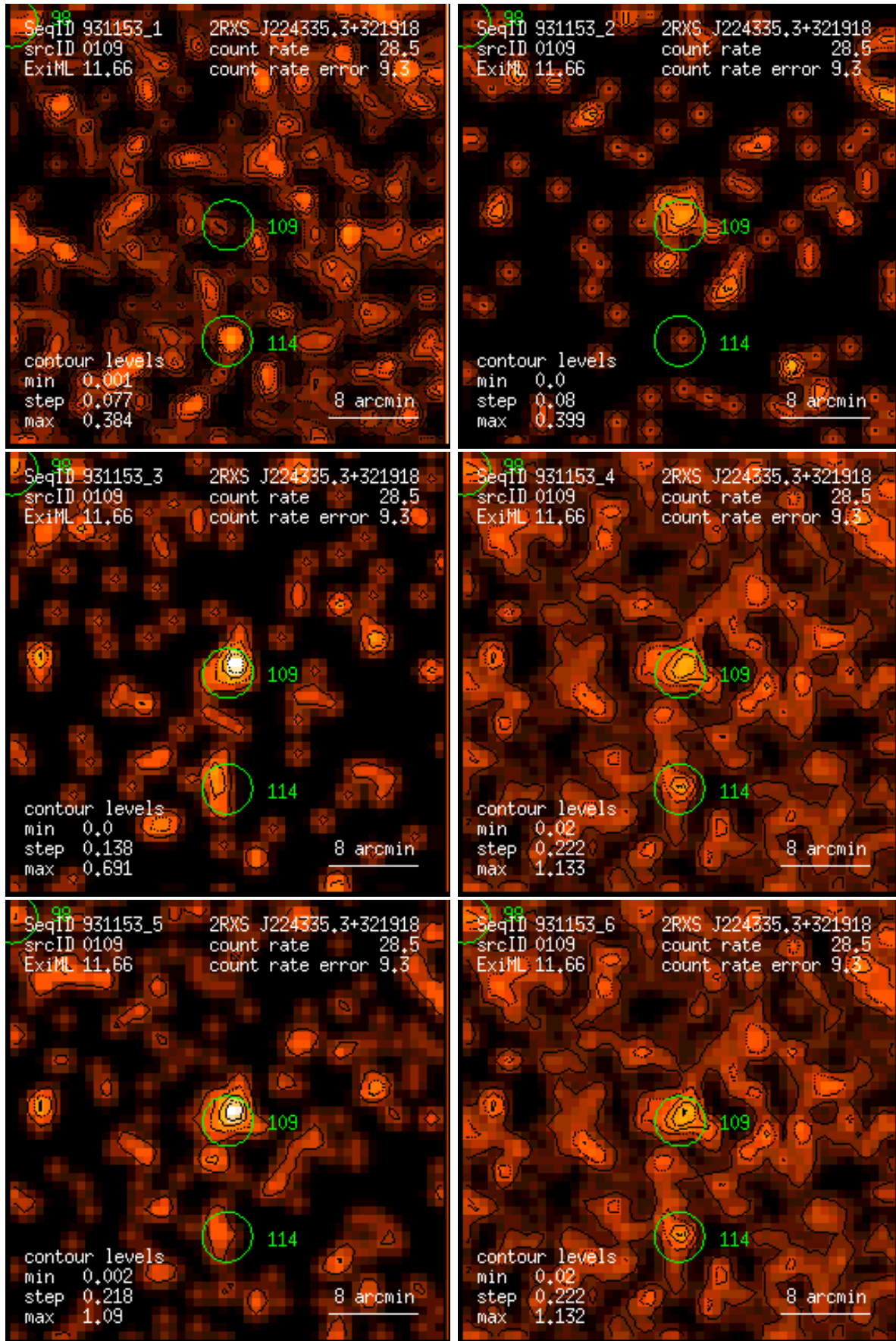
Figure 109: RASS 931153: detection 0109: band rate images, Gaussian filter: (1) PSPC channels 11 – 41, (2) 52 – 90, (3) 91 – 201, (4) 11 – 235, (5) 52 – 201, (6) 11 – 201. Broad band rates in counts/ks. Band rate contour levels in counts/ks/arcmin 2 .
