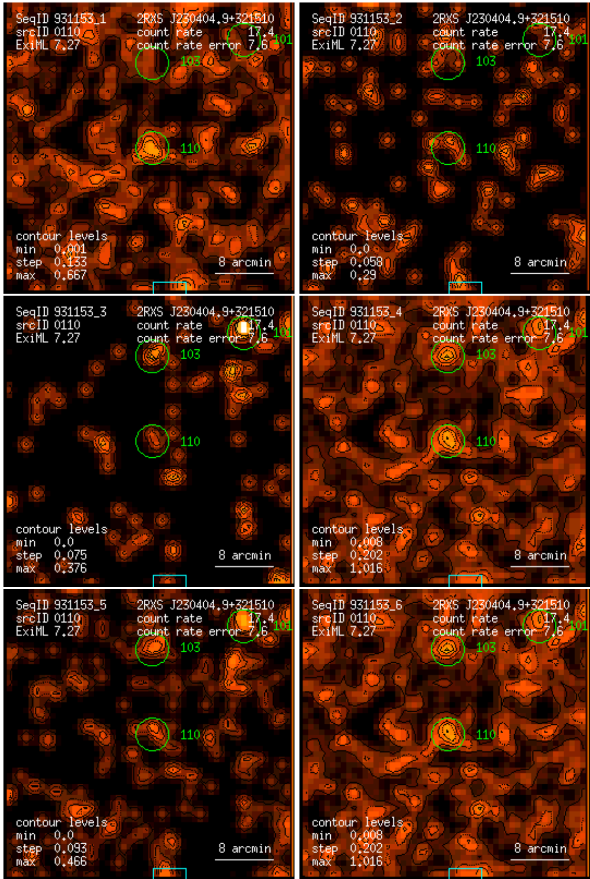
Figure 110: RASS 931153: detection 0110: band rate images, Gaussian filter: (1) PSPC channels 11 – 41, (2) 52 – 90, (3) 91 – 201, (4) 11 – 235, (5) 52 – 201, (6) 11 – 201. Broad band rates in counts/ks. Band rate contour levels in counts/ks/arcmin 2 .
