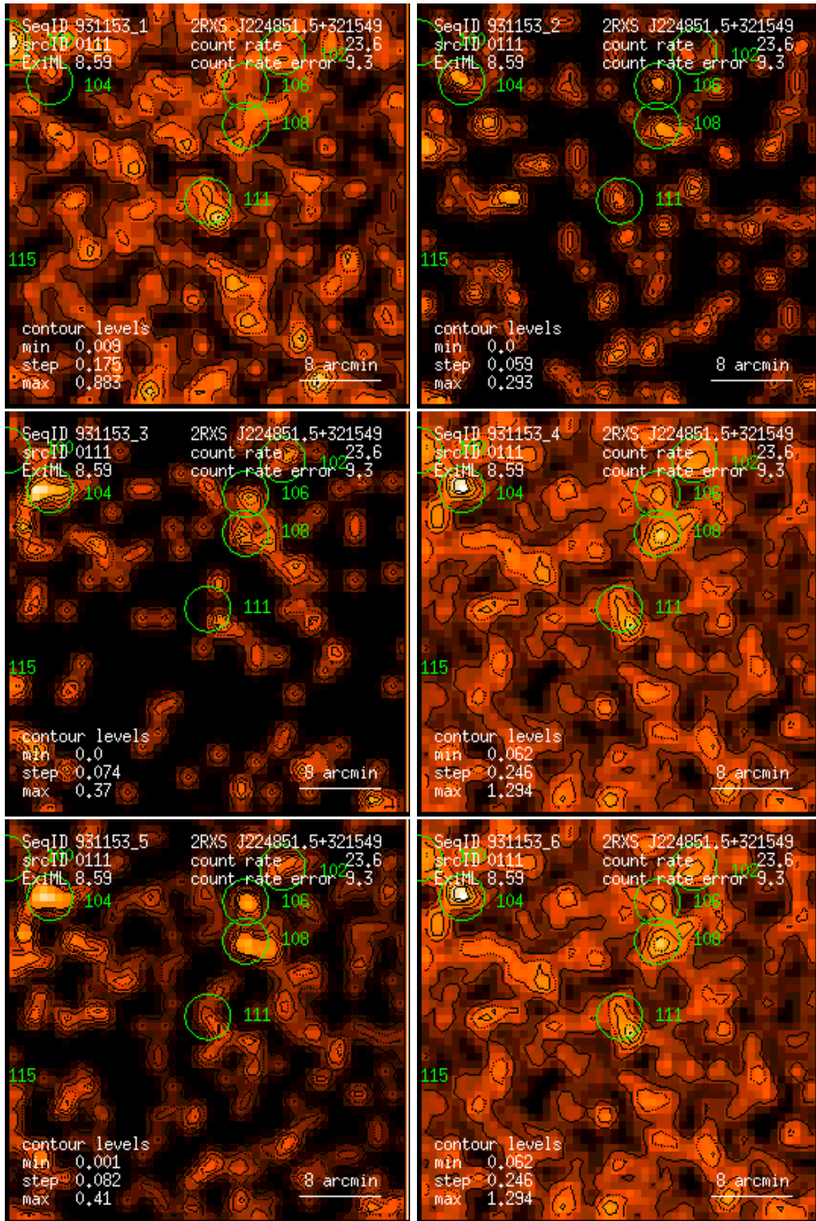
Figure 111: RASS 931153: detection 0111: band rate images, Gaussian filter: (1) PSPC channels 11 – 41, (2) 52 – 90, (3) 91 – 201, (4) 11 – 235, (5) 52 – 201, (6) 11 – 201. Broad band rates in counts/ks. Band rate contour levels in counts/ks/arcmin 2 .
