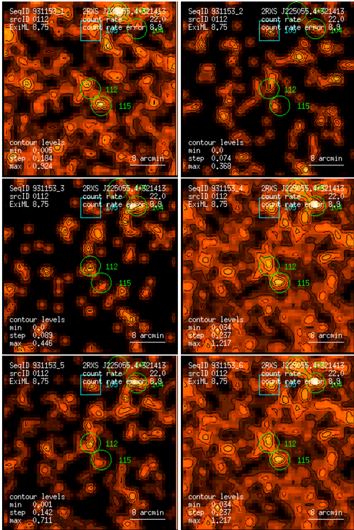
Figure 112: RASS 931153: detection 0112: band rate images, Gaussian filter: (1) PSPC channels 11 – 41, (2) 52 – 90, (3) 91 – 201, (4) 11 – 235, (5) 52 – 201, (6) 11 – 201. Broad band rates in counts/ks. Band rate contour levels in counts/ks/arcmin 2 .
