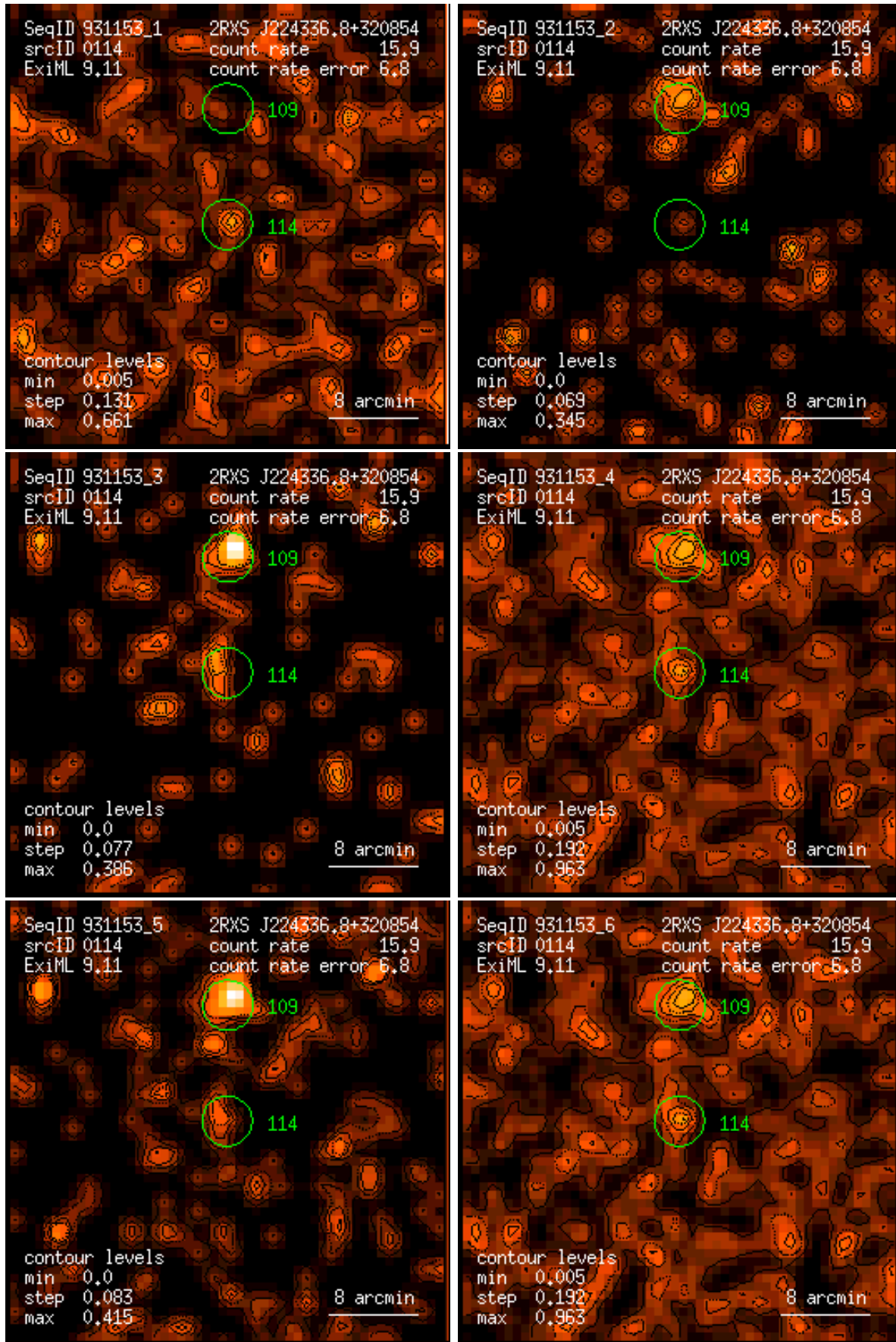
Figure 114: RASS 931153: detection 0114: band rate images, Gaussian filter: (1) PSPC channels 11 – 41, (2) 52 – 90, (3) 91 – 201, (4) 11 – 235, (5) 52 – 201, (6) 11 – 201. Broad band rates in counts/ks. Band rate contour levels in counts/ks/arcmin 2 .
