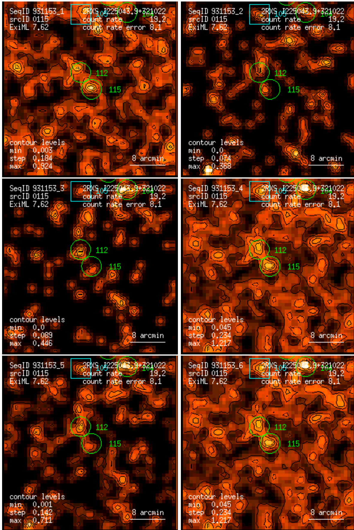
Figure 115: RASS 931153: detection 0115: band rate images, Gaussian filter: (1) PSPC channels 11 – 41, (2) 52 – 90, (3) 91 – 201, (4) 11 – 235, (5) 52 – 201, (6) 11 – 201. Broad band rates in counts/ks. Band rate contour levels in counts/ks/arcmin 2 .
