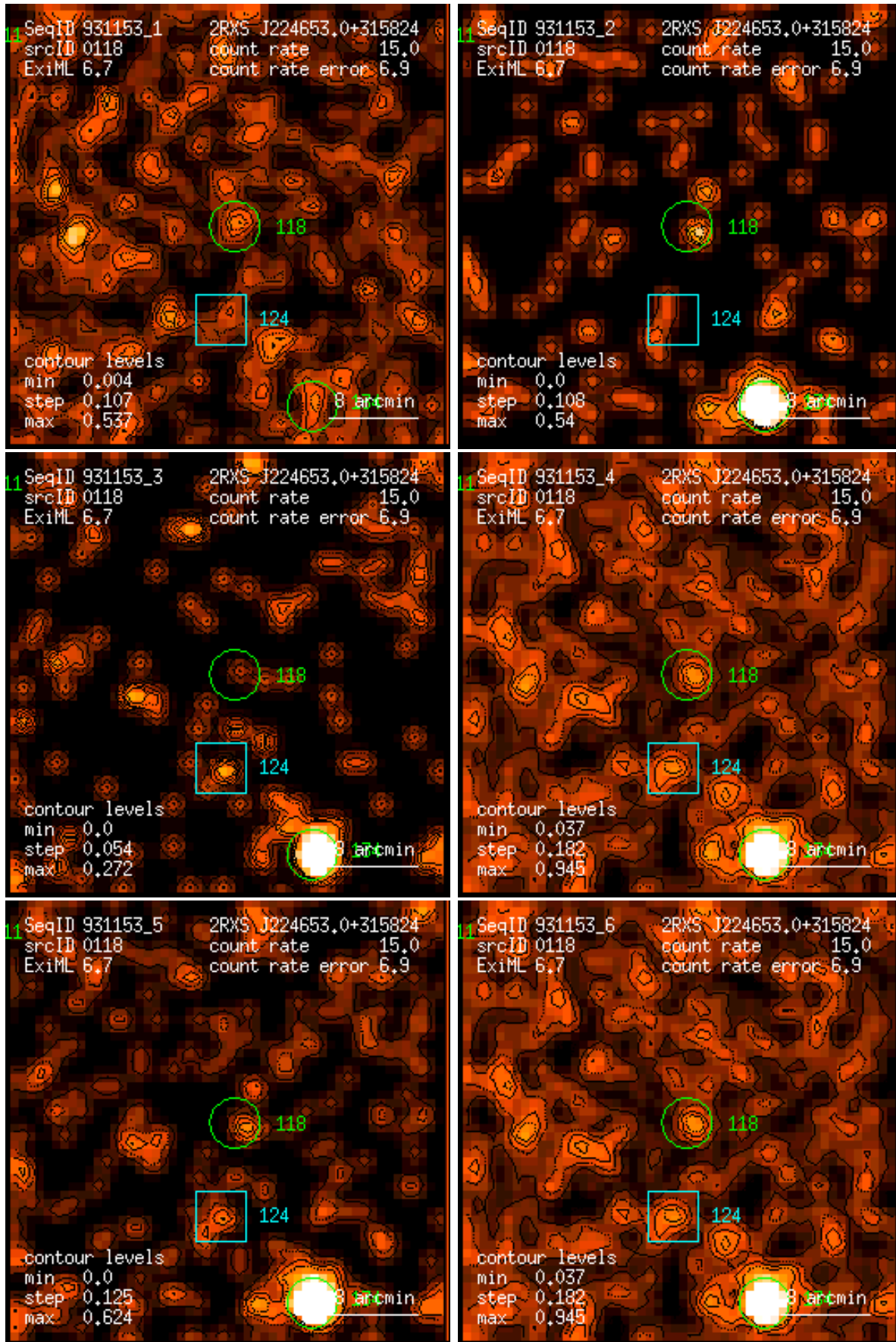
Figure 118: RASS 931153: detection 0118: band rate images, Gaussian filter: (1) PSPC channels 11 – 41, (2) 52 – 90, (3) 91 – 201, (4) 11 – 235, (5) 52 – 201, (6) 11 – 201. Broad band rates in counts/ks. Band rate contour levels in counts/ks/arcmin 2 .
