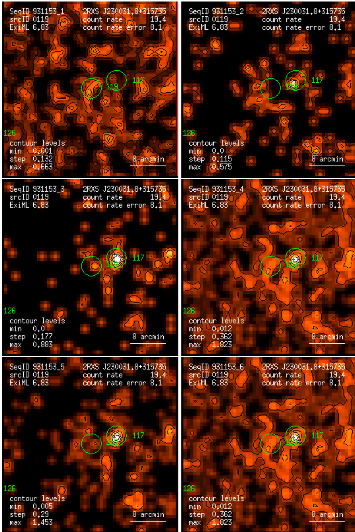
Figure 119: RASS 931153: detection 0119: band rate images, Gaussian filter: (1) PSPC channels 11 – 41, (2) 52 – 90, (3) 91 – 201, (4) 11 – 235, (5) 52 – 201, (6) 11 – 201. Broad band rates in counts/ks. Band rate contour levels in counts/ks/arcmin 2 .
