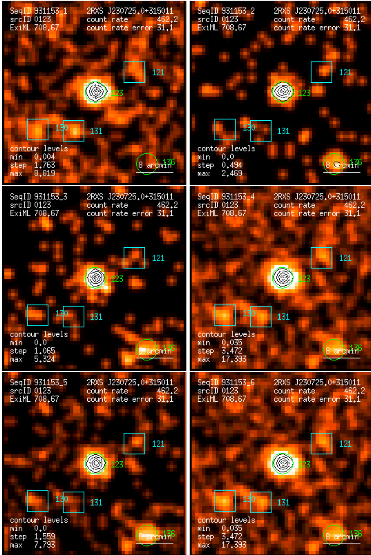
Figure 123: RASS 931153: detection 0123: band rate images, Gaussian filter: (1) PSPC channels 11 – 41, (2) 52 – 90, (3) 91 – 201, (4) 11 – 235, (5) 52 – 201, (6) 11 – 201. Broad band rates in counts/ks. Band rate contour levels in counts/ks/arcmin 2 .
