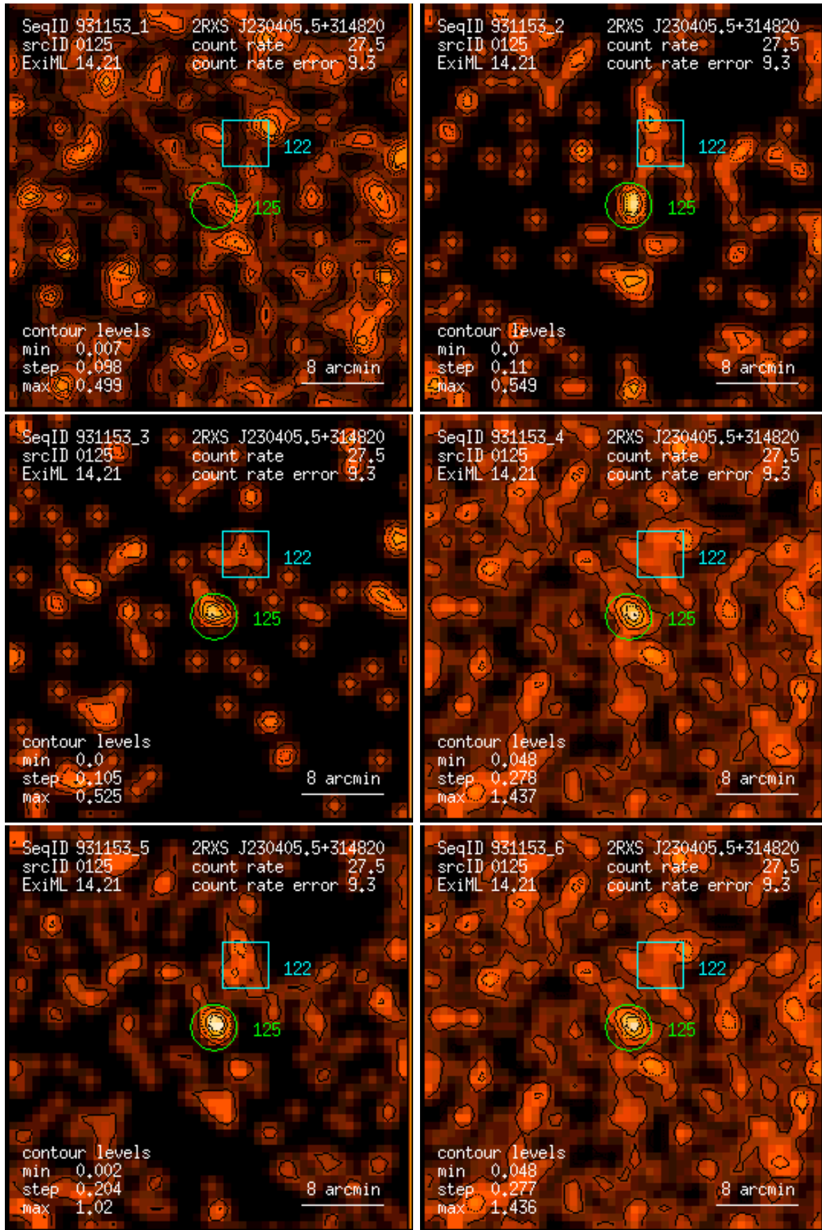
Figure 125: RASS 931153: detection 0125: band rate images, Gaussian filter: (1) PSPC channels 11 – 41, (2) 52 – 90, (3) 91 – 201, (4) 11 – 235, (5) 52 – 201, (6) 11 – 201. Broad band rates in counts/ks. Band rate contour levels in counts/ks/arcmin 2 .
