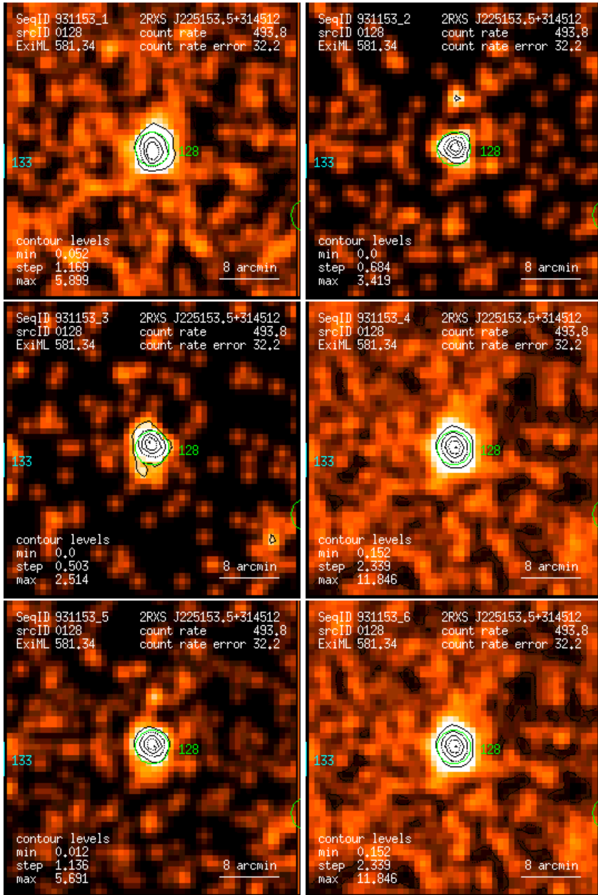
Figure 128: RASS 931153: detection 0128: band rate images, Gaussian filter: (1) PSPC channels 11 – 41, (2) 52 – 90, (3) 91 – 201, (4) 11 – 235, (5) 52 – 201, (6) 11 – 201. Broad band rates in counts/ks. Band rate contour levels in counts/ks/arcmin 2 .
