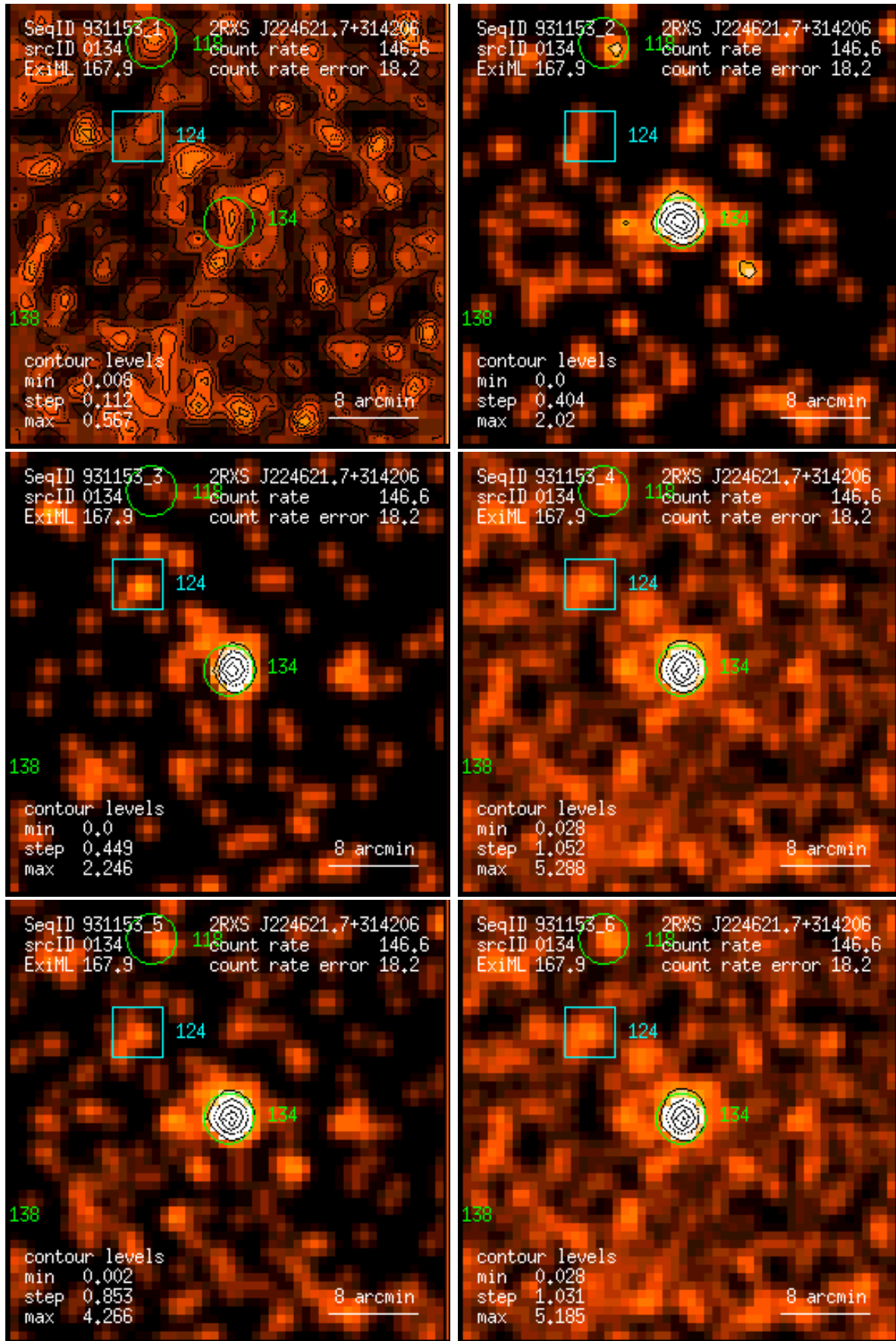
Figure 134: RASS 931153: detection 0134: band rate images, Gaussian filter: (1) PSPC channels 11 – 41, (2) 52 – 90, (3) 91 – 201, (4) 11 – 235, (5) 52 – 201, (6) 11 – 201. Broad band rates in counts/ks. Band rate contour levels in counts/ks/arcmin 2 .
