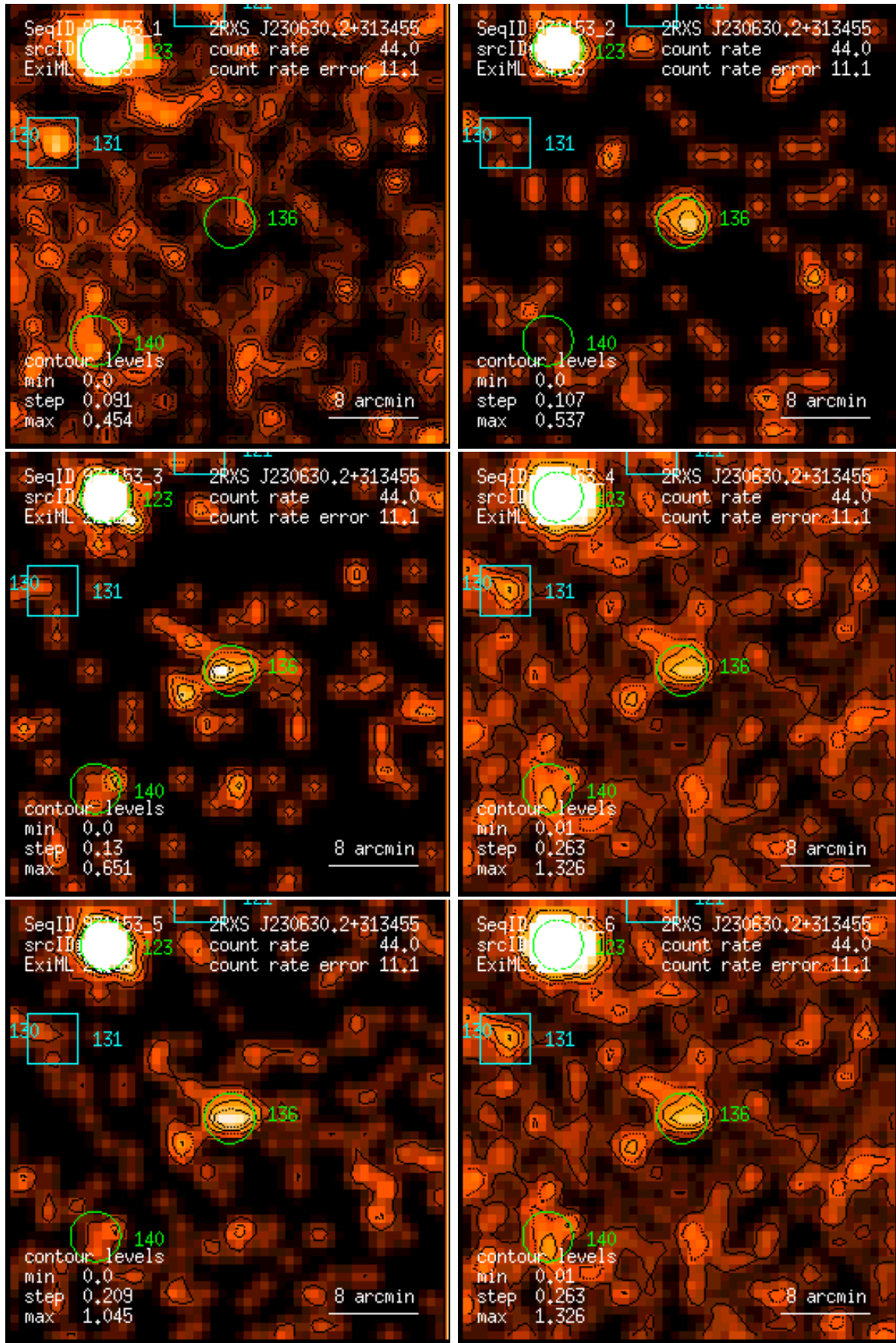
Figure 136: RASS 931153: detection 0136: band rate images, Gaussian filter: (1) PSPC channels 11 – 41, (2) 52 – 90, (3) 91 – 201, (4) 11 – 235, (5) 52 – 201, (6) 11 – 201. Broad band rates in counts/ks. Band rate contour levels in counts/ks/arcmin 2 .
