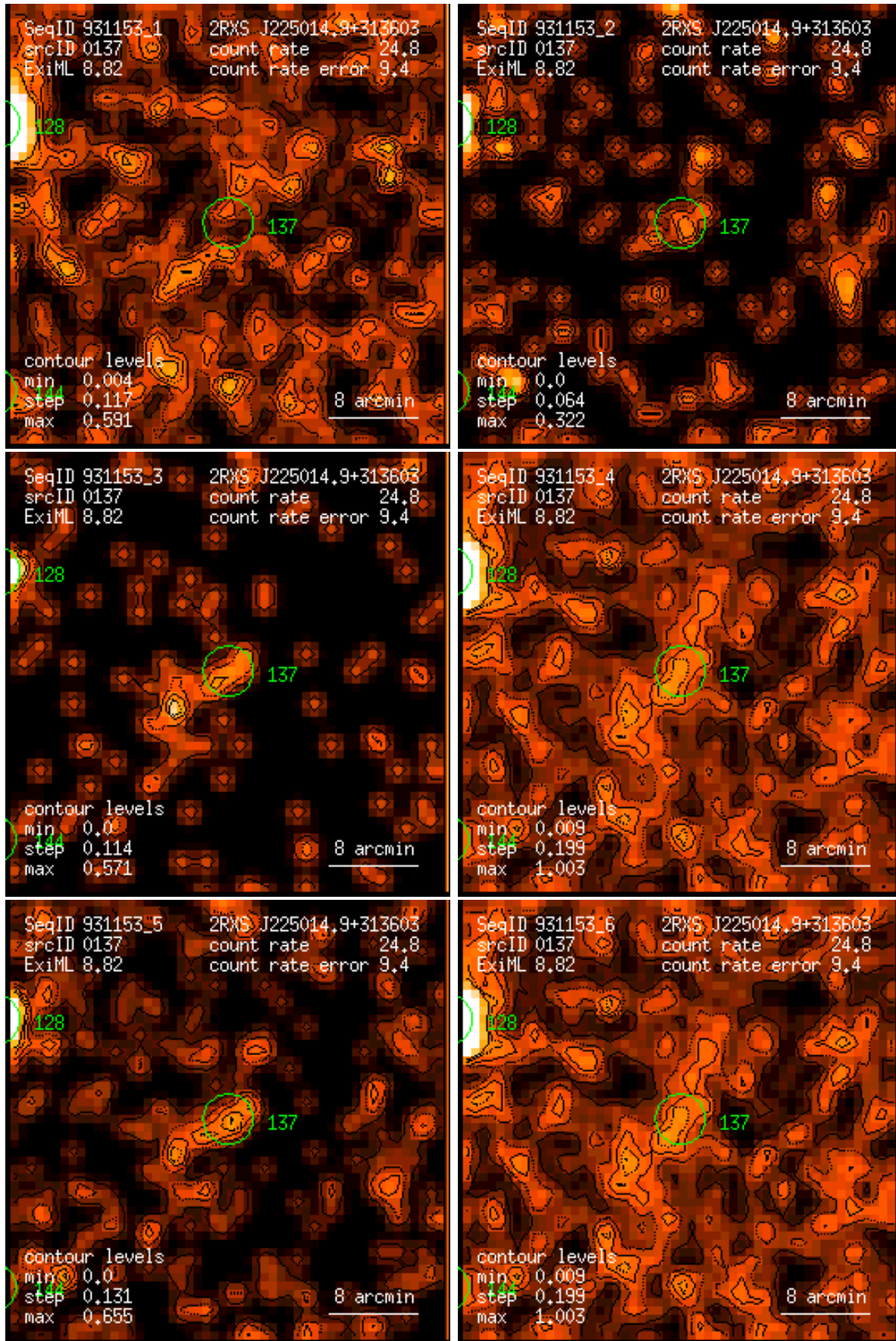
Figure 137: RASS 931153: detection 0137: band rate images, Gaussian filter: (1) PSPC channels 11 – 41, (2) 52 – 90, (3) 91 – 201, (4) 11 – 235, (5) 52 – 201, (6) 11 – 201. Broad band rates in counts/ks. Band rate contour levels in counts/ks/arcmin 2 .
