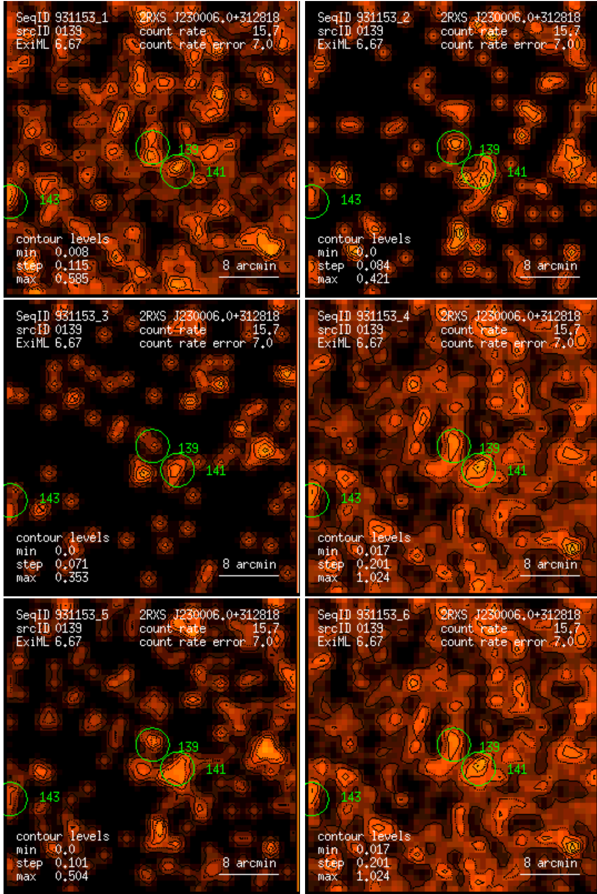
Figure 139: RASS 931153: detection 0139: band rate images, Gaussian filter: (1) PSPC channels 11 – 41, (2) 52 – 90, (3) 91 – 201, (4) 11 – 235, (5) 52 – 201, (6) 11 – 201. Broad band rates in counts/ks. Band rate contour levels in counts/ks/arcmin 2 .
