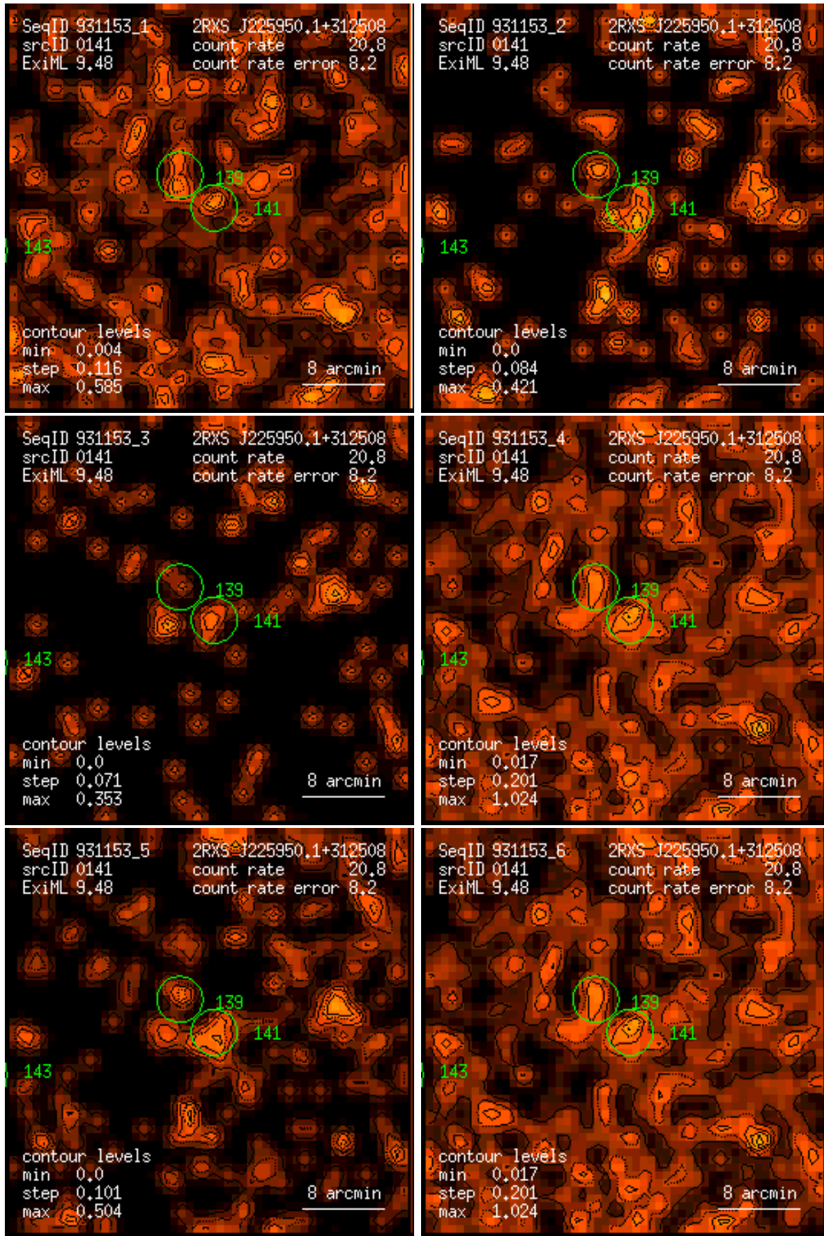
Figure 141: RASS 931153: detection 0141: band rate images, Gaussian filter: (1) PSPC channels 11 – 41, (2) 52 – 90, (3) 91 – 201, (4) 11 – 235, (5) 52 – 201, (6) 11 – 201. Broad band rates in counts/ks. Band rate contour levels in counts/ks/arcmin 2 .
