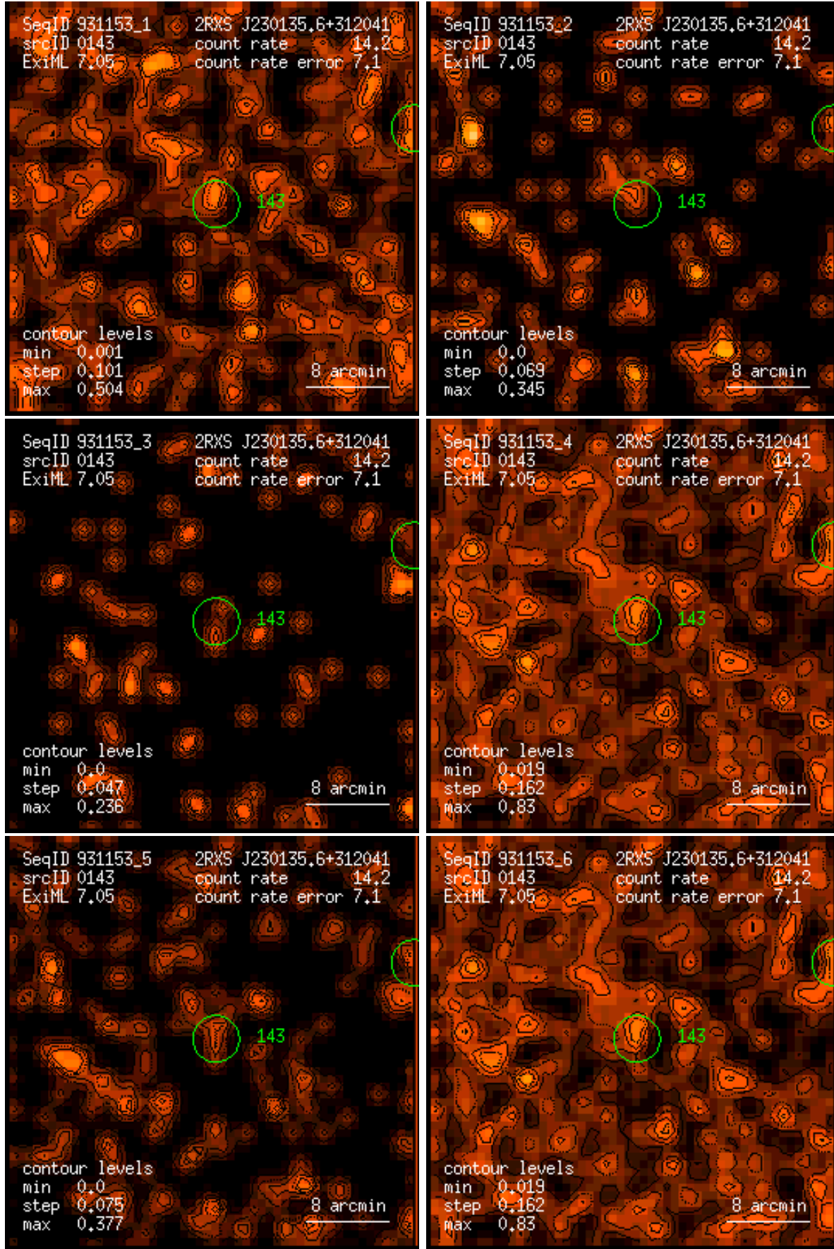
Figure 143: RASS 931153: detection 0143: band rate images, Gaussian filter: (1) PSPC channels 11 – 41, (2) 52 – 90, (3) 91 – 201, (4) 11 – 235, (5) 52 – 201, (6) 11 – 201. Broad band rates in counts/ks. Band rate contour levels in counts/ks/arcmin 2 .
