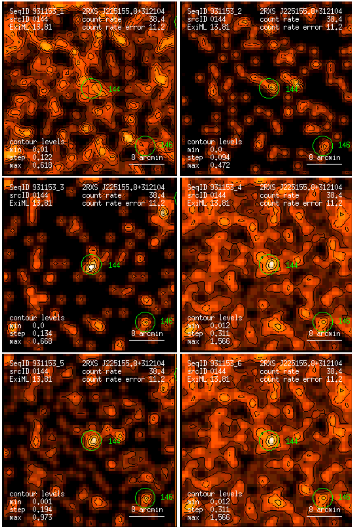
Figure 144: RASS 931153: detection 0144: band rate images, Gaussian filter: (1) PSPC channels 11 – 41, (2) 52 – 90, (3) 91 – 201, (4) 11 – 235, (5) 52 – 201, (6) 11 – 201. Broad band rates in counts/ks. Band rate contour levels in counts/ks/arcmin 2 .
