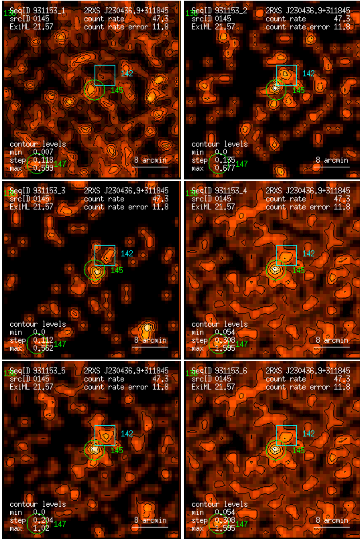
Figure 145: RASS 931153: detection 0145: band rate images, Gaussian filter: (1) PSPC channels 11 – 41, (2) 52 – 90, (3) 91 – 201, (4) 11 – 235, (5) 52 – 201, (6) 11 – 201. Broad band rates in counts/ks. Band rate contour levels in counts/ks/arcmin 2 .
