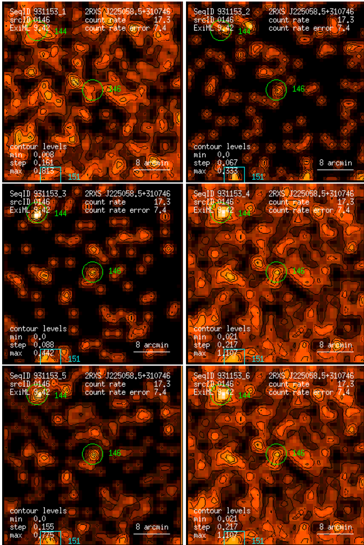
Figure 146: RASS 931153: detection 0146: band rate images, Gaussian filter: (1) PSPC channels 11 – 41, (2) 52 – 90, (3) 91 – 201, (4) 11 – 235, (5) 52 – 201, (6) 11 – 201. Broad band rates in counts/ks. Band rate contour levels in counts/ks/arcmin 2 .
