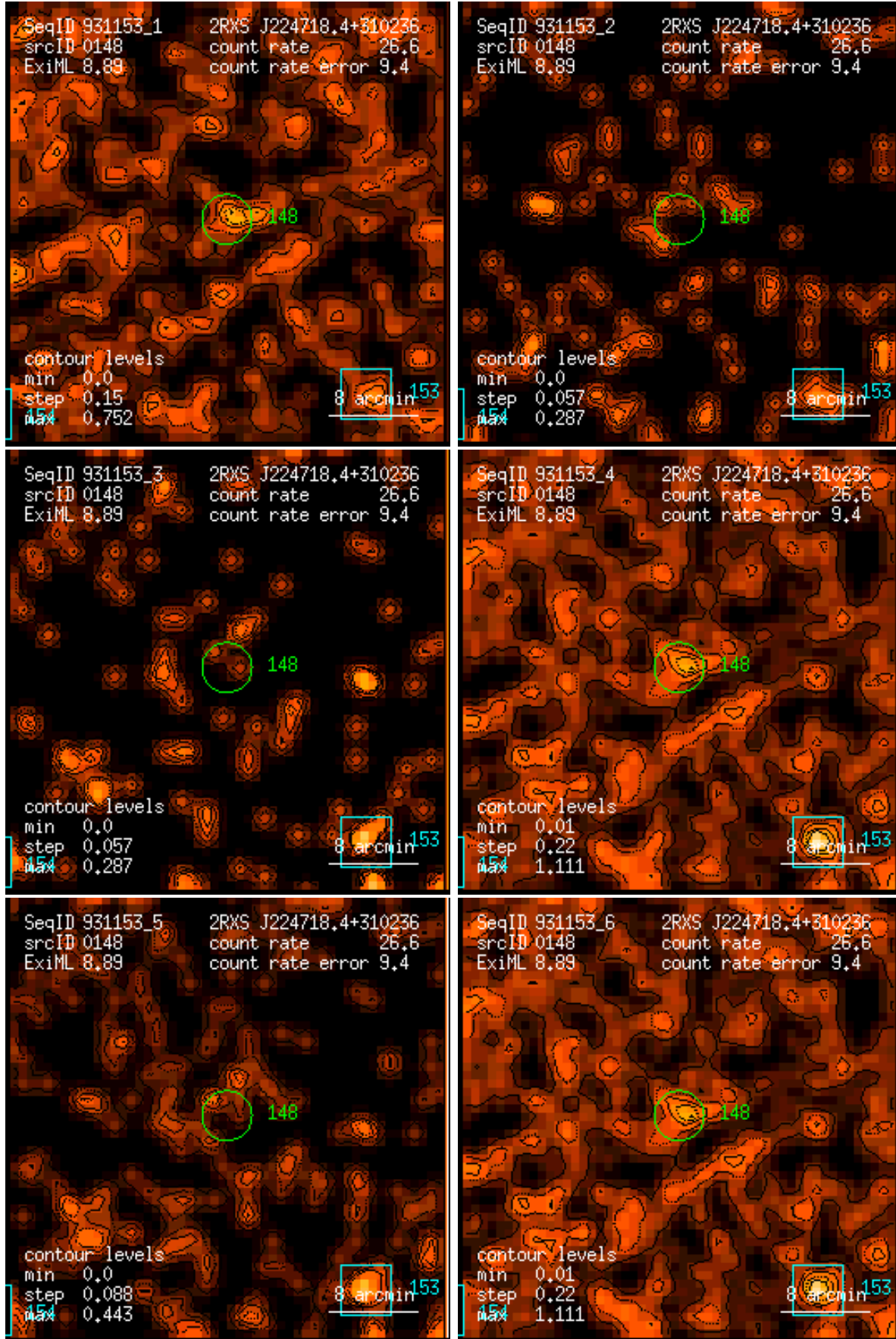
Figure 148: RASS 931153: detection 0148: band rate images, Gaussian filter: (1) PSPC channels 11 – 41, (2) 52 – 90, (3) 91 – 201, (4) 11 – 235, (5) 52 – 201, (6) 11 – 201. Broad band rates in counts/ks. Band rate contour levels in counts/ks/arcmin 2 .
