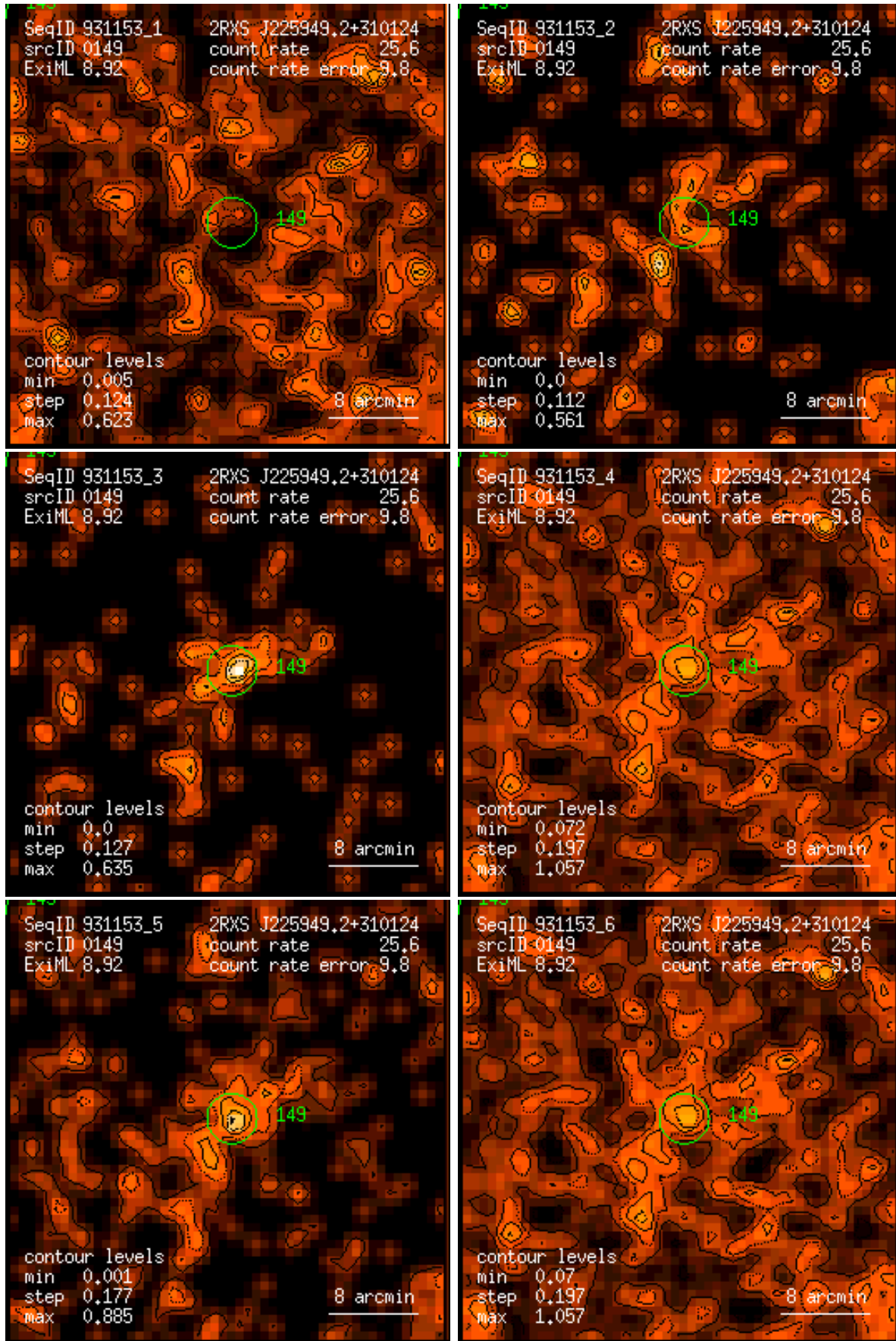
Figure 149: RASS 931153: detection 0149: band rate images, Gaussian filter: (1) PSPC channels 11 – 41, (2) 52 – 90, (3) 91 – 201, (4) 11 – 235, (5) 52 – 201, (6) 11 – 201. Broad band rates in counts/ks. Band rate contour levels in counts/ks/arcmin 2 .
