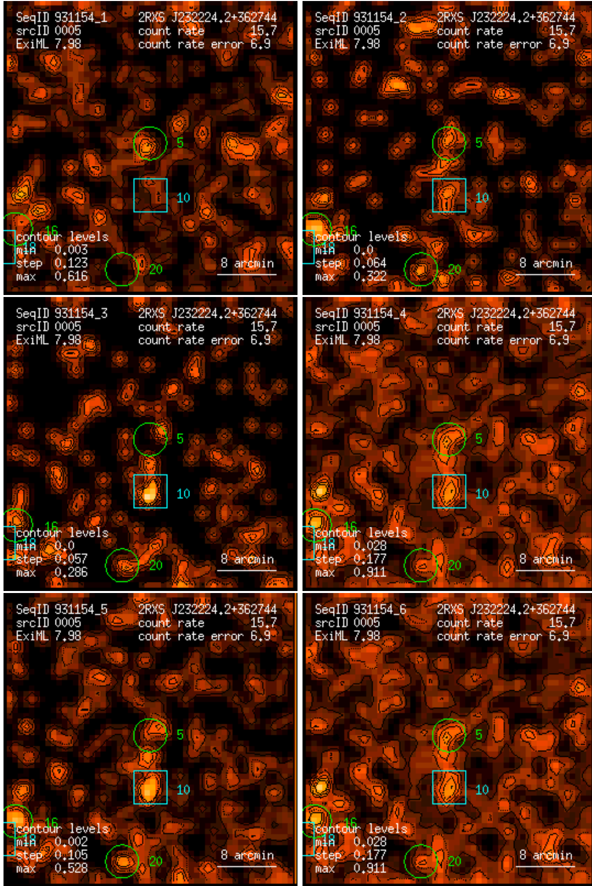
Figure 5: RASS 931154: detection 0005: band rate images, Gaussian filter: (1) PSPC channels 11 – 41, (2) 52 – 90, (3) 91 – 201, (4) 11 – 235, (5) 52 – 201, (6) 11 – 201. Broad band rates in counts/ks. Band rate contour levels in counts/ks/arcmin 2 .
