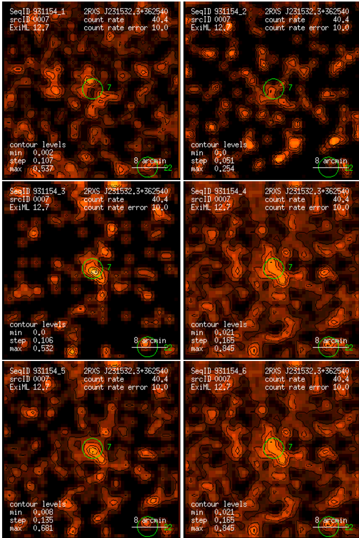
Figure 7: RASS 931154: detection 0007: band rate images, Gaussian filter: (1) PSPC channels 11 – 41, (2) 52 – 90, (3) 91 – 201, (4) 11 – 235, (5) 52 – 201, (6) 11 – 201. Broad band rates in counts/ks. Band rate contour levels in counts/ks/arcmin 2 .
