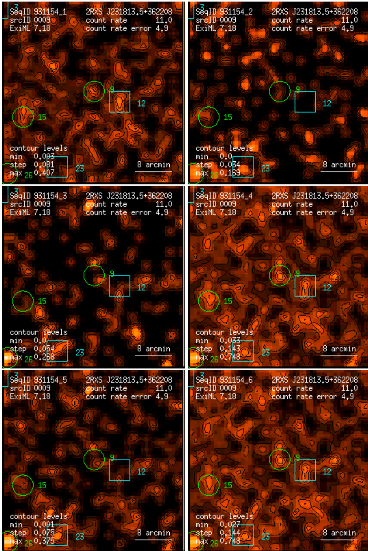
Figure 9: RASS 931154: detection 0009: band rate images, Gaussian filter: (1) PSPC channels 11 – 41, (2) 52 – 90, (3) 91 – 201, (4) 11 – 235, (5) 52 – 201, (6) 11 – 201. Broad band rates in counts/ks. Band rate contour levels in counts/ks/arcmin 2 .
