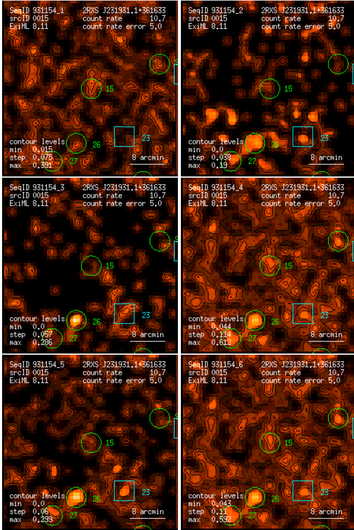
Figure 15: RASS 931154: detection 0015: band rate images, Gaussian filter: (1) PSPC channels 11 – 41, (2) 52 – 90, (3) 91 – 201, (4) 11 – 235, (5) 52 – 201, (6) 11 – 201. Broad band rates in counts/ks. Band rate contour levels in counts/ks/arcmin 2 .
