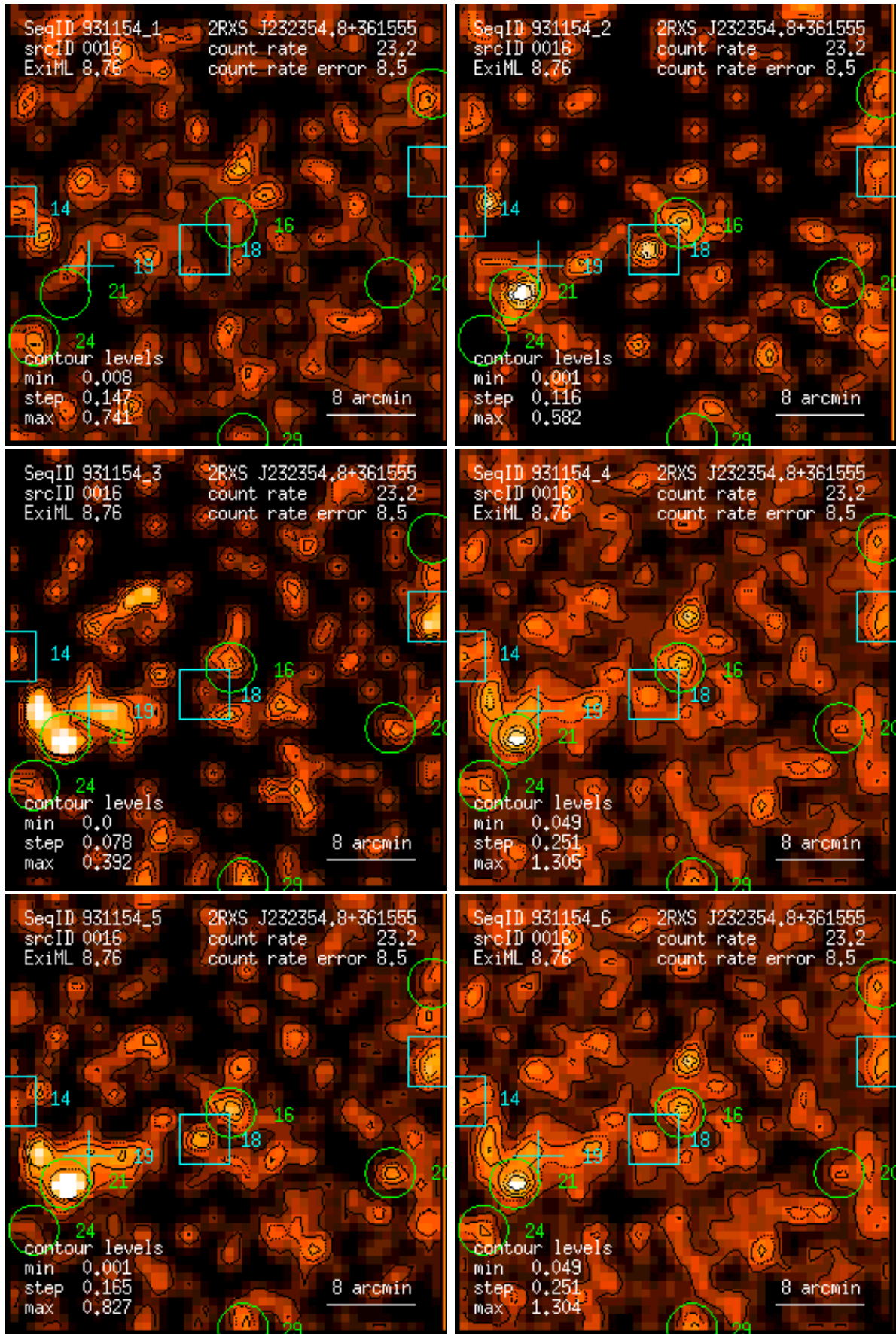
Figure 16: RASS 931154: detection 0016: band rate images, Gaussian filter: (1) PSPC channels 11 – 41, (2) 52 – 90, (3) 91 – 201, (4) 11 – 235, (5) 52 – 201, (6) 11 – 201. Broad band rates in counts/ks. Band rate contour levels in counts/ks/arcmin 2 .
