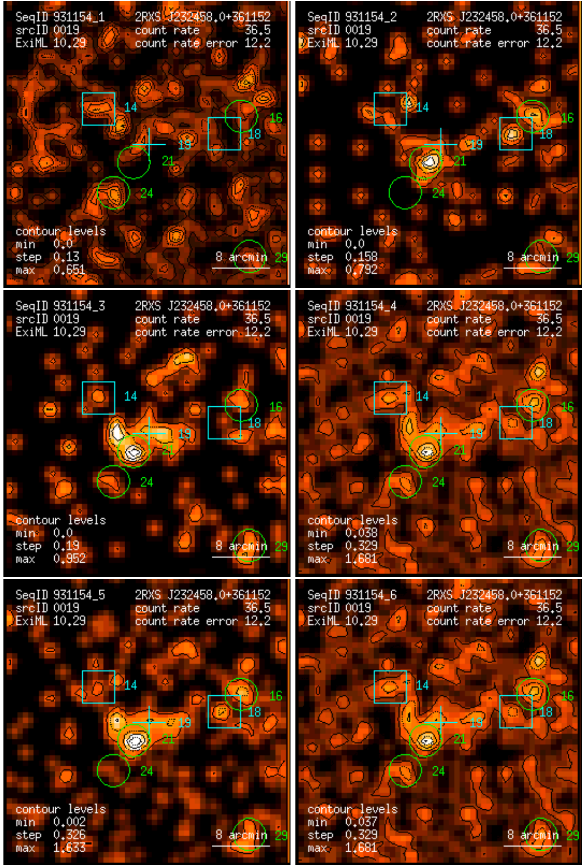
Figure 19: RASS 931154: detection 0019: band rate images, Gaussian filter: (1) PSPC channels 11 – 41, (2) 52 – 90, (3) 91 – 201, (4) 11 – 235, (5) 52 – 201, (6) 11 – 201. Broad band rates in counts/ks. Band rate contour levels in counts/ks/arcmin 2 .
