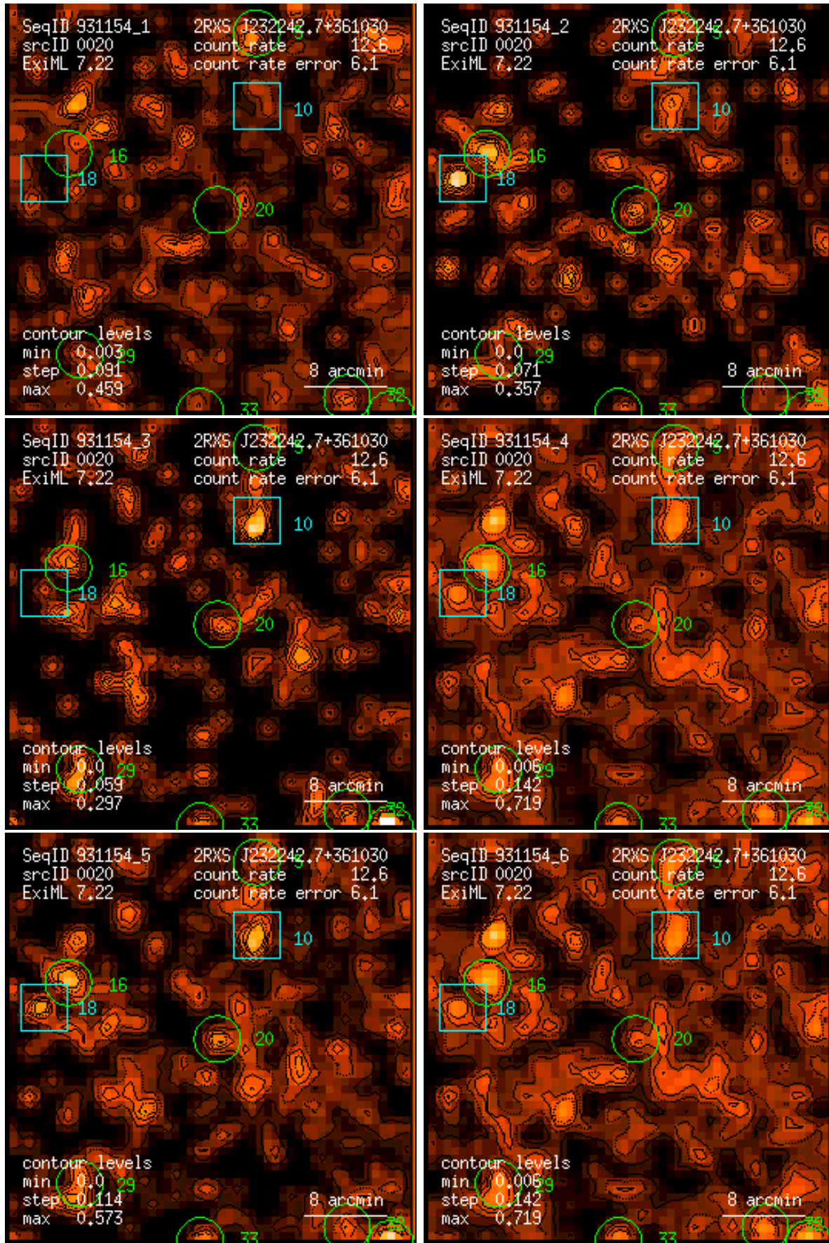
Figure 20: RASS 931154: detection 0020: band rate images, Gaussian filter: (1) PSPC channels 11 – 41, (2) 52 – 90, (3) 91 – 201, (4) 11 – 235, (5) 52 – 201, (6) 11 – 201. Broad band rates in counts/ks. Band rate contour levels in counts/ks/arcmin 2 .
