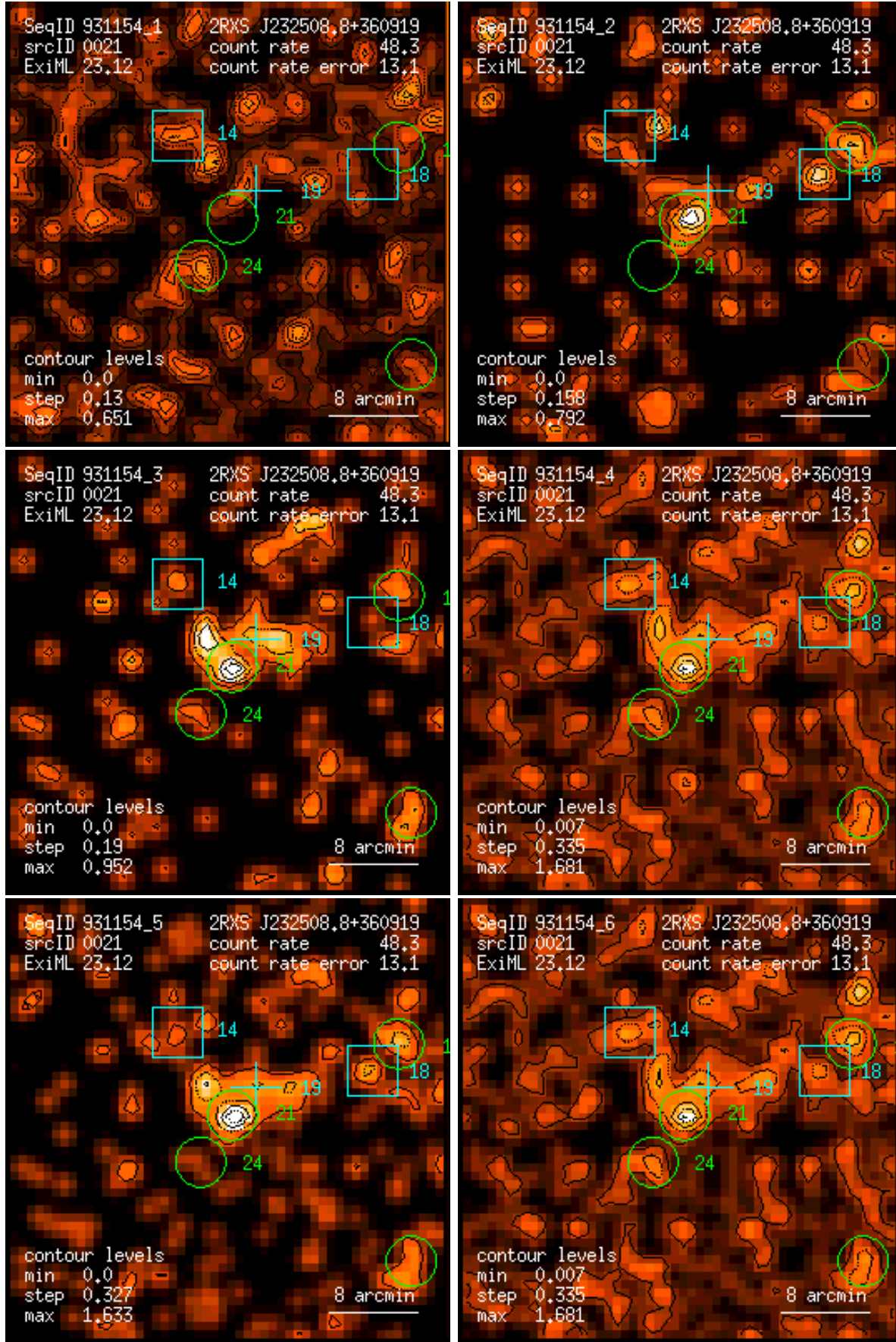
Figure 21: RASS 931154: detection 0021: band rate images, Gaussian filter: (1) PSPC channels 11 – 41, (2) 52 – 90, (3) 91 – 201, (4) 11 – 235, (5) 52 – 201, (6) 11 – 201. Broad band rates in counts/ks. Band rate contour levels in counts/ks/arcmin 2 .
