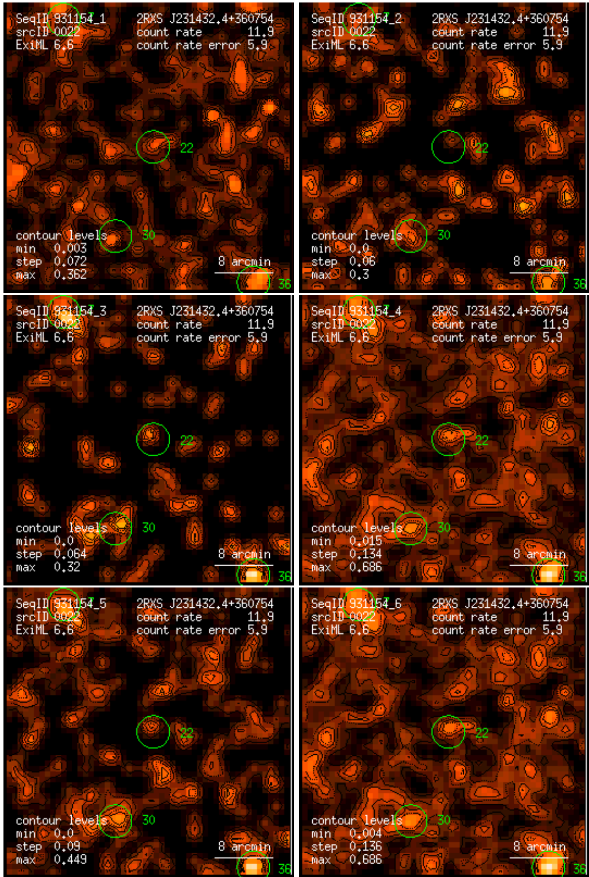
Figure 22: RASS 931154: detection 0022: band rate images, Gaussian filter: (1) PSPC channels 11 – 41, (2) 52 – 90, (3) 91 – 201, (4) 11 – 235, (5) 52 – 201, (6) 11 – 201. Broad band rates in counts/ks. Band rate contour levels in counts/ks/arcmin 2 .
