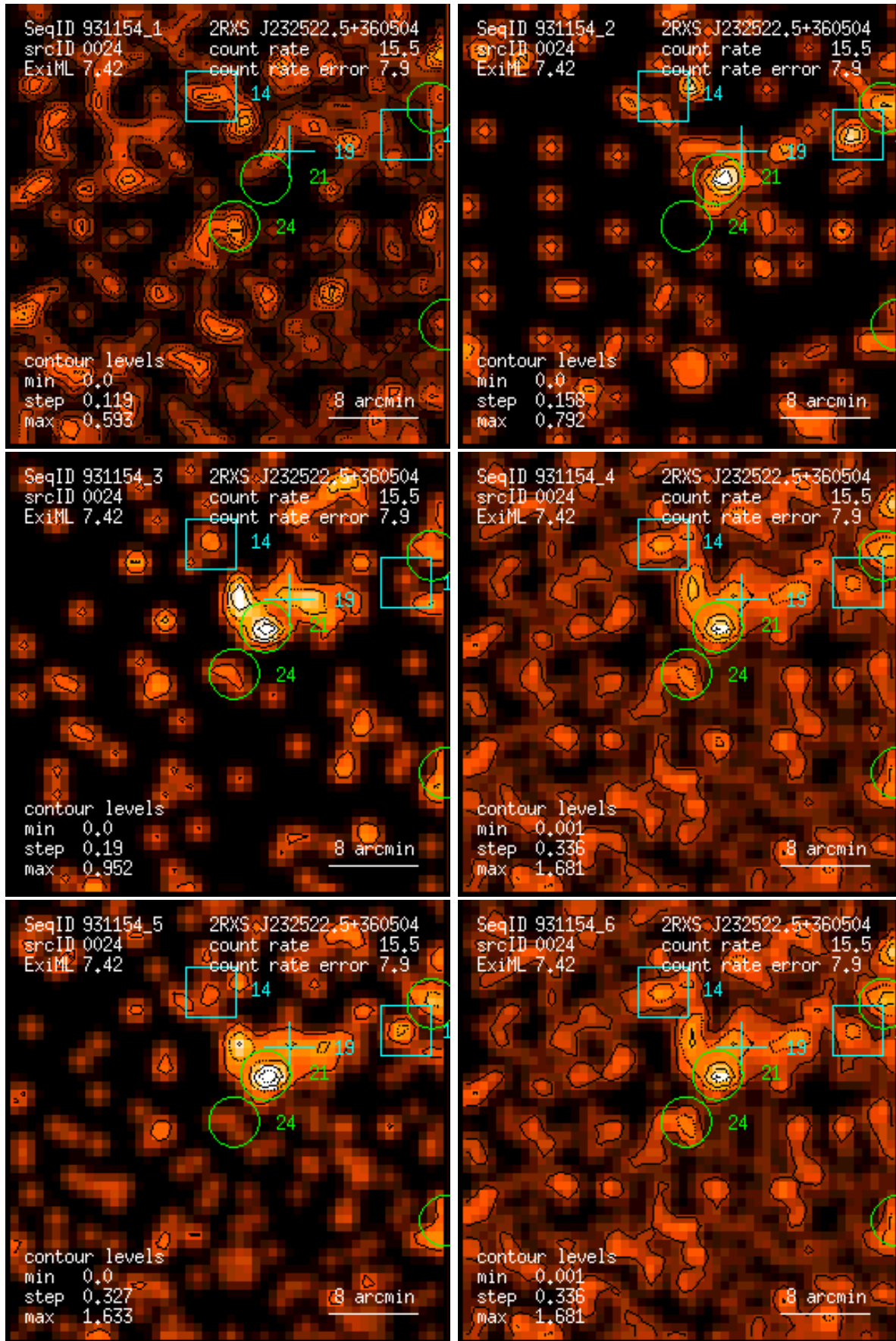
Figure 24: RASS 931154: detection 0024: band rate images, Gaussian filter: (1) PSPC channels 11 – 41, (2) 52 – 90, (3) 91 – 201, (4) 11 – 235, (5) 52 – 201, (6) 11 – 201. Broad band rates in counts/ks. Band rate contour levels in counts/ks/arcmin 2 .
