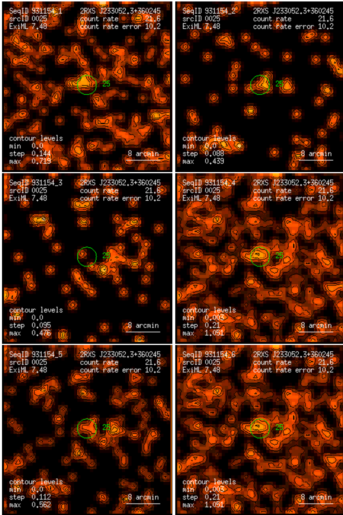
Figure 25: RASS 931154: detection 0025: band rate images, Gaussian filter: (1) PSPC channels 11 – 41, (2) 52 – 90, (3) 91 – 201, (4) 11 – 235, (5) 52 – 201, (6) 11 – 201. Broad band rates in counts/ks. Band rate contour levels in counts/ks/arcmin 2 .
