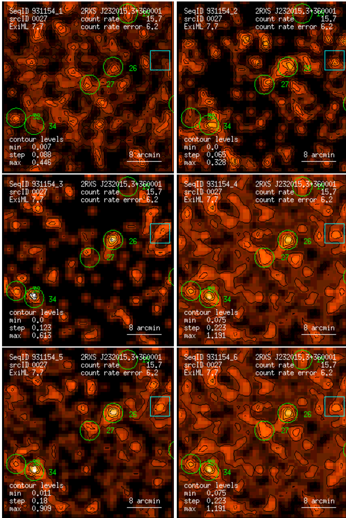
Figure 27: RASS 931154: detection 0027: band rate images, Gaussian filter: (1) PSPC channels 11 – 41, (2) 52 – 90, (3) 91 – 201, (4) 11 – 235, (5) 52 – 201, (6) 11 – 201. Broad band rates in counts/ks. Band rate contour levels in counts/ks/arcmin 2 .
