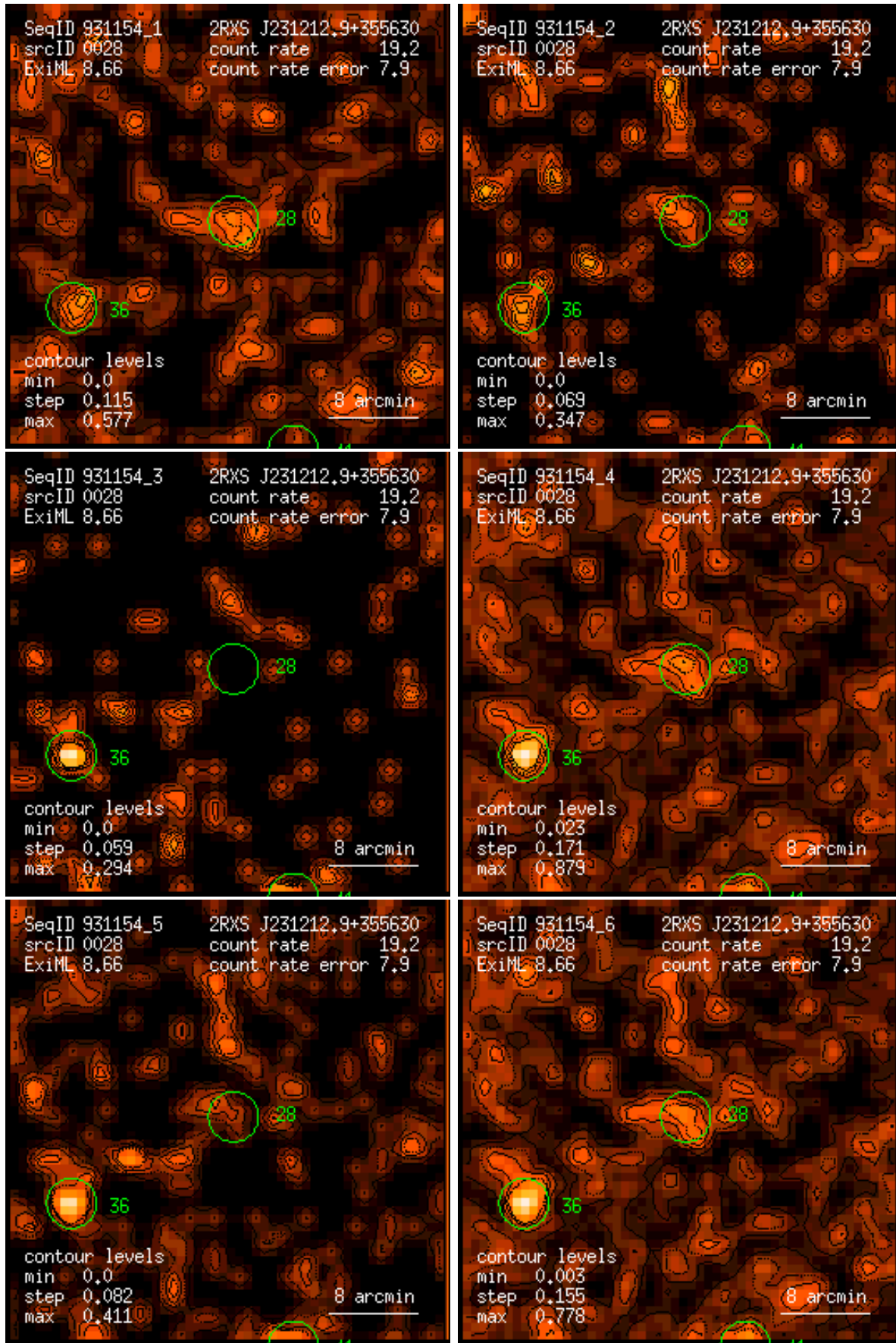
Figure 28: RASS 931154: detection 0028: band rate images, Gaussian filter: (1) PSPC channels 11 – 41, (2) 52 – 90, (3) 91 – 201, (4) 11 – 235, (5) 52 – 201, (6) 11 – 201. Broad band rates in counts/ks. Band rate contour levels in counts/ks/arcmin 2 .
