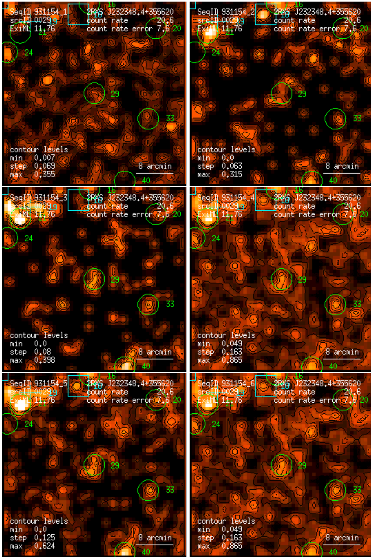
Figure 29: RASS 931154: detection 0029: band rate images, Gaussian filter: (1) PSPC channels 11 – 41, (2) 52 – 90, (3) 91 – 201, (4) 11 – 235, (5) 52 – 201, (6) 11 – 201. Broad band rates in counts/ks. Band rate contour levels in counts/ks/arcmin 2 .
