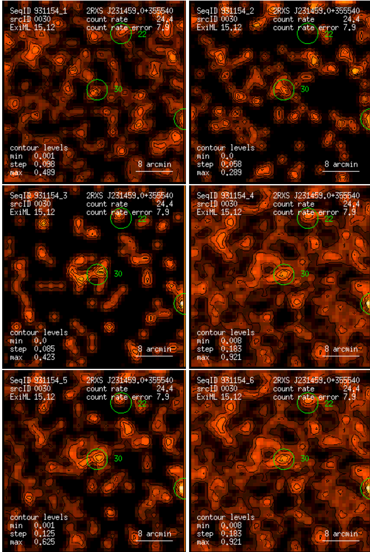
Figure 30: RASS 931154: detection 0030: band rate images, Gaussian filter: (1) PSPC channels 11 – 41, (2) 52 – 90, (3) 91 – 201, (4) 11 – 235, (5) 52 – 201, (6) 11 – 201. Broad band rates in counts/ks. Band rate contour levels in counts/ks/arcmin 2 .
