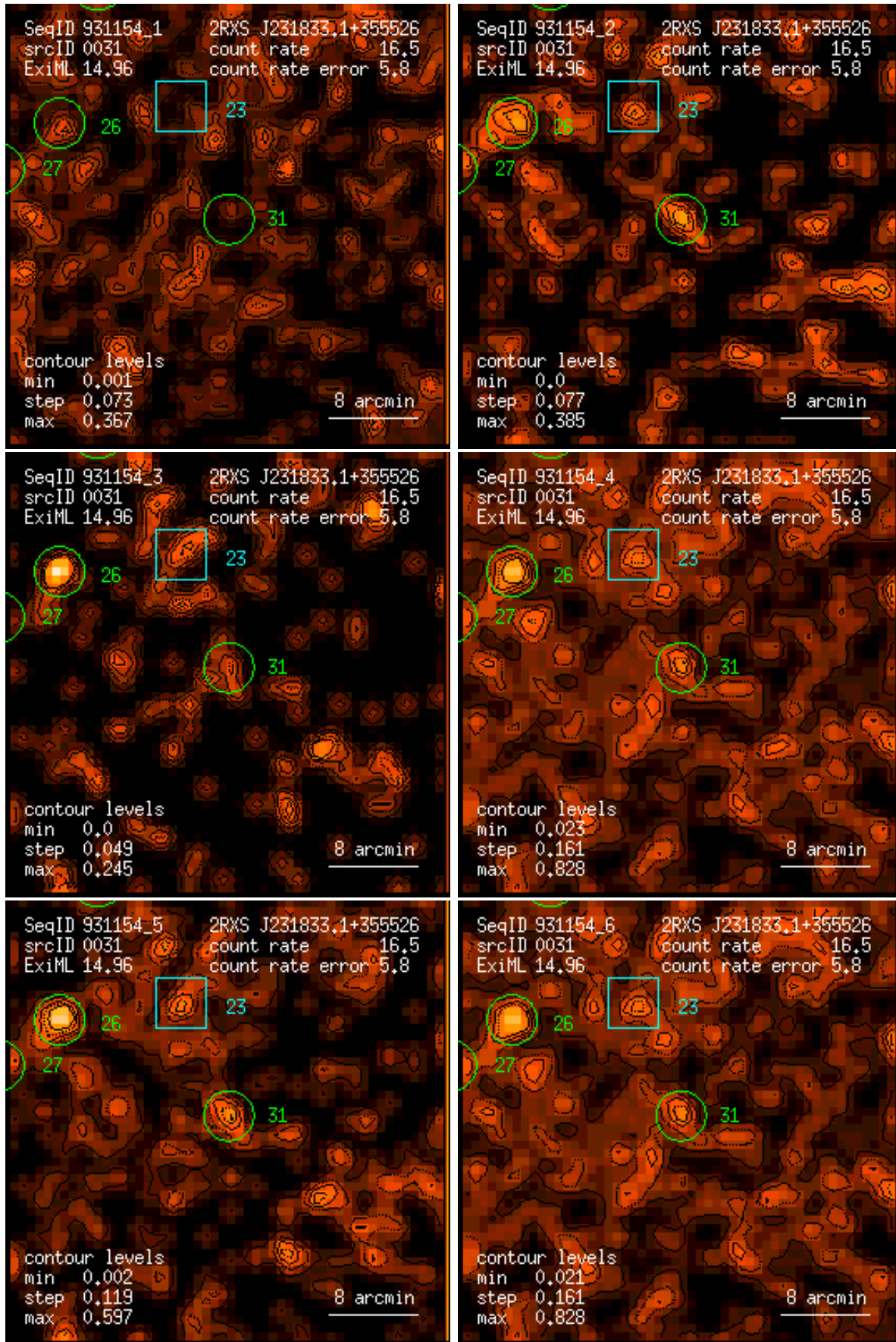
Figure 31: RASS 931154: detection 0031: band rate images, Gaussian filter: (1) PSPC channels 11 – 41, (2) 52 – 90, (3) 91 – 201, (4) 11 – 235, (5) 52 – 201, (6) 11 – 201. Broad band rates in counts/ks. Band rate contour levels in counts/ks/arcmin 2 .
