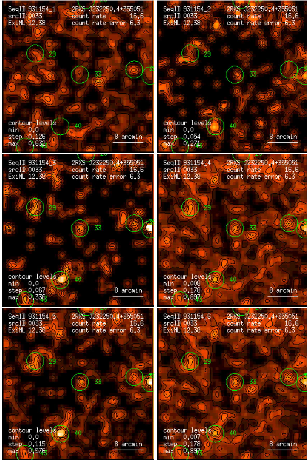
Figure 33: RASS 931154: detection 0033: band rate images, Gaussian filter: (1) PSPC channels 11 – 41, (2) 52 – 90, (3) 91 – 201, (4) 11 – 235, (5) 52 – 201, (6) 11 – 201. Broad band rates in counts/ks. Band rate contour levels in counts/ks/arcmin 2 .
