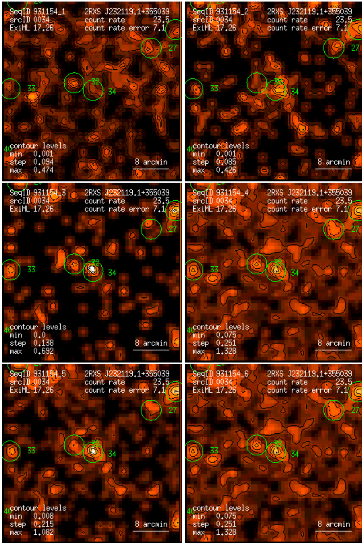
Figure 34: RASS 931154: detection 0034: band rate images, Gaussian filter: (1) PSPC channels 11 – 41, (2) 52 – 90, (3) 91 – 201, (4) 11 – 235, (5) 52 – 201, (6) 11 – 201. Broad band rates in counts/ks. Band rate contour levels in counts/ks/arcmin 2 .
