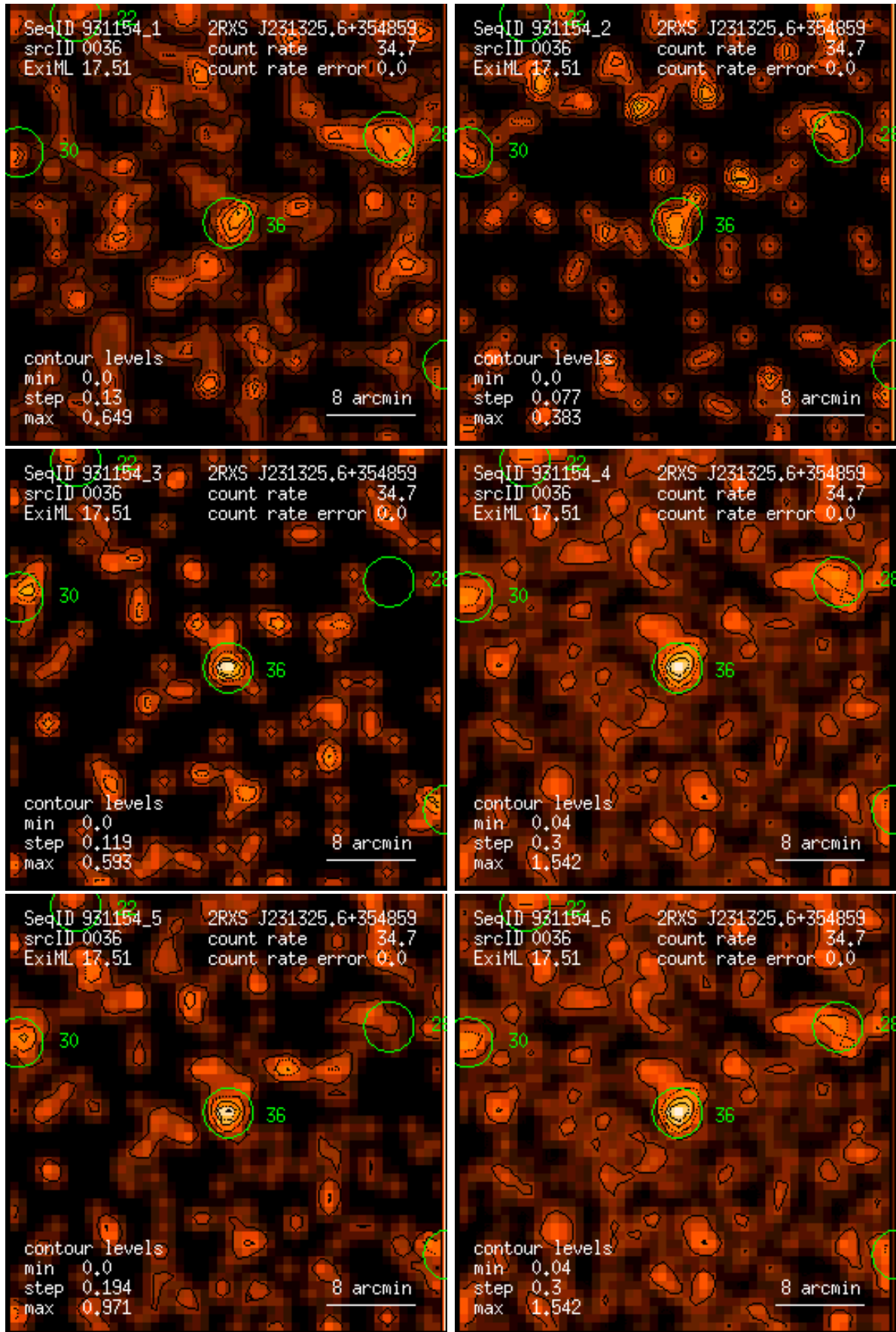
Figure 36: RASS 931154: detection 0036: band rate images, Gaussian filter: (1) PSPC channels 11 – 41, (2) 52 – 90, (3) 91 – 201, (4) 11 – 235, (5) 52 – 201, (6) 11 – 201. Broad band rates in counts/ks. Band rate contour levels in counts/ks/arcmin 2 .
