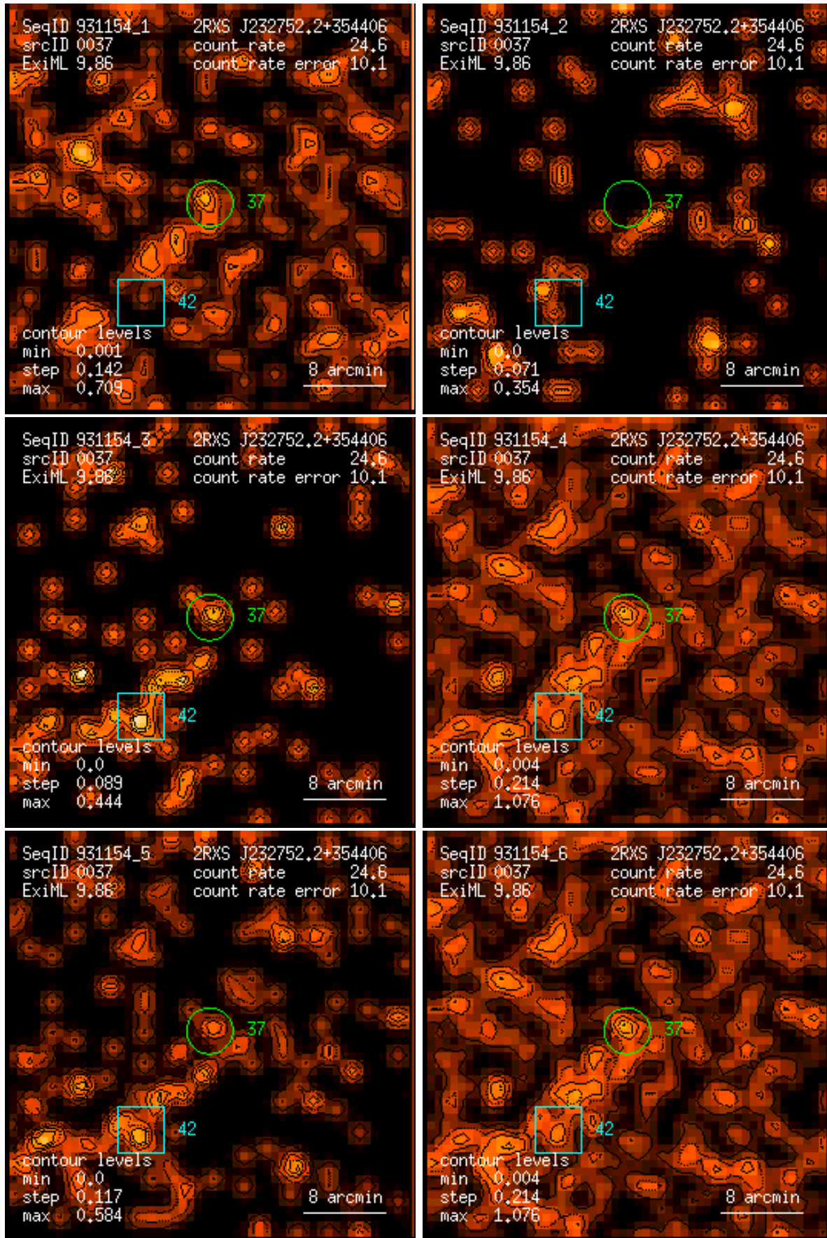
Figure 37: RASS 931154: detection 0037: band rate images, Gaussian filter: (1) PSPC channels 11 – 41, (2) 52 – 90, (3) 91 – 201, (4) 11 – 235, (5) 52 – 201, (6) 11 – 201. Broad band rates in counts/ks. Band rate contour levels in counts/ks/arcmin 2 .
