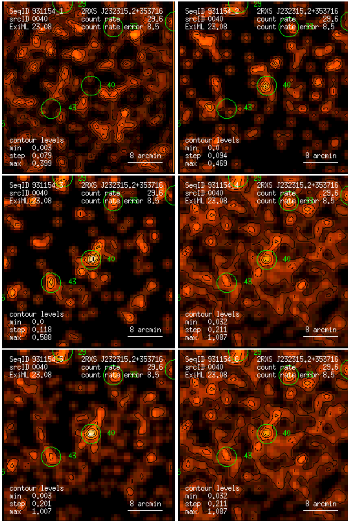
Figure 40: RASS 931154: detection 0040: band rate images, Gaussian filter: (1) PSPC channels 11 – 41, (2) 52 – 90, (3) 91 – 201, (4) 11 – 235, (5) 52 – 201, (6) 11 – 201. Broad band rates in counts/ks. Band rate contour levels in counts/ks/arcmin 2 .
