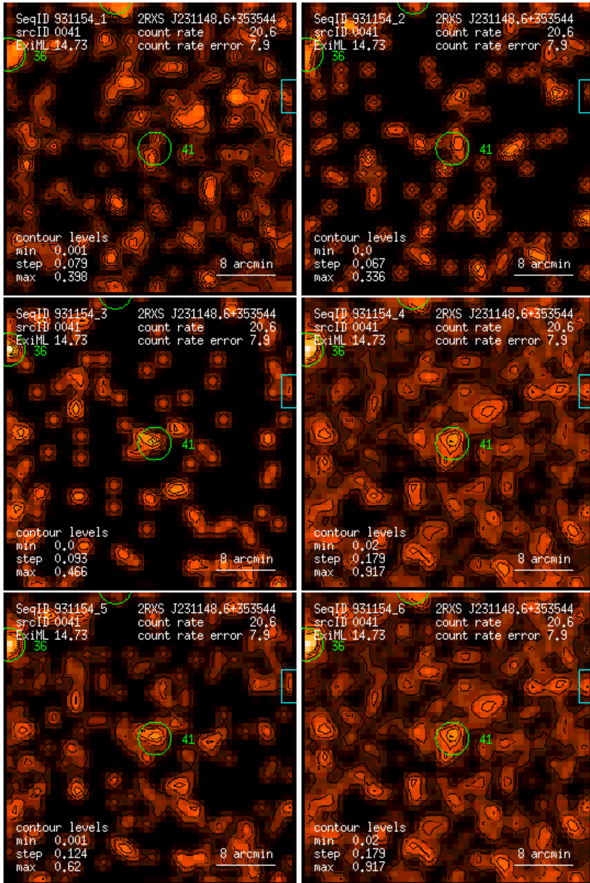
Figure 41: RASS 931154: detection 0041: band rate images, Gaussian filter: (1) PSPC channels 11 – 41, (2) 52 – 90, (3) 91 – 201, (4) 11 – 235, (5) 52 – 201, (6) 11 – 201. Broad band rates in counts/ks. Band rate contour levels in counts/ks/arcmin 2 .
